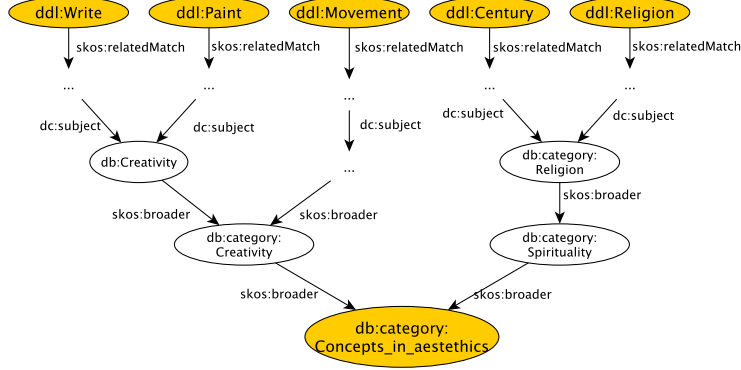
Figure 2: Example of the Linked Data graph traversal. The search starts at the top with the words in \mathcal{C}_{y1} . The walks they share in the graph are collected and then evaluated in order to find the most suitable ones.
