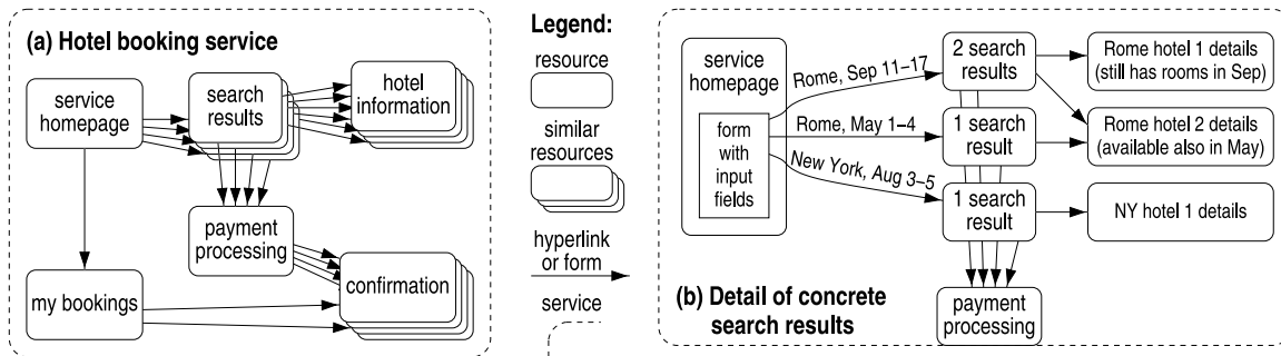
Fig. 4. Structure of an example RESTful hotel reservation service: (a) showing types of resources, (b) showing details of example search results resources that make up a part of the service.
