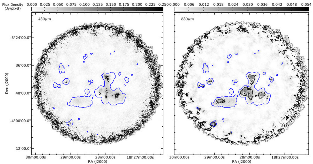
Figure 1. SCUBA-2 450 \mu\text{m} (left) and 850 \mu\text{m} (right) data. Contours show 5\sigma and 15\sigma levels in both cases: levels are at 0.082, 0.25 \text{Jy 4 arcsec}^{-1} pixel and 0.011, 0.033 \text{Jy 6 arcsec}^{-1} pixel at 450 \mu\text{m} and 850 \mu\text{m} , respectively. The blue outer contour shows the data reduction mask for the region, based on Herschel 500 \mu\text{m} observations. Noise levels increase towards the edges of the map on account of the mapping method outlined in Section 2.1.
