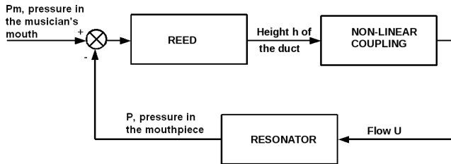
FIG. 1. Model of a self-sustained wind instrument 6,19 .
