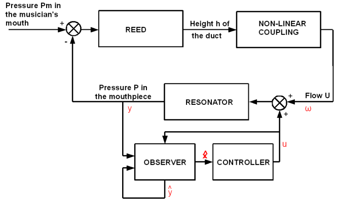
FIG. 2. Model of a self-sustained wind instrument with control system. w , y and u_s are defined in eq.(24). \hat{y} and \hat{\mathbf{x}} are the observer estimations of y and \mathbf{x} .
