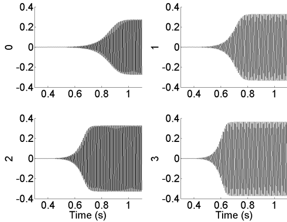
FIG. 6. Attack transients of the self-sustained oscillating system with \gamma = 0.4 . Top left : Case 0 (uncontrolled). Top right : Case 1 ( f_1 = 120\text{Hz} ). Bottom left : Case 2 ( \xi_{1_n} reduced by a factor of 2). Bottom right : Case 3 ( f_1 = 120\text{Hz} and \xi_{1_n} reduced by a factor of 2).
