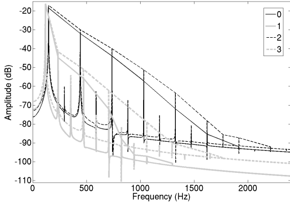
FIG. 5. Enveloped sound spectra of the self-sustained oscillating system in cases 0 (uncontrolled, solid black line), 1 ( f_1 = 120\text{Hz} , solid grey line), 2 ( \xi_{1_n} reduced by a factor of 2, dash black line) and 3 ( f_1 = 120\text{Hz} and \xi_{1_n} reduced by a factor of 2, dash grey line), with \gamma = 0.4 .
