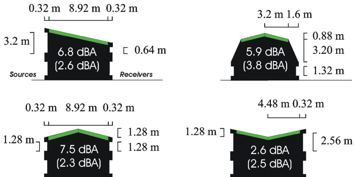
Figure 7. Green-roof road traffic noise insertion losses for different building shapes in a street-canyon setup, referenced to identical building shapes but with perfectly reflecting roofs. The values in between brackets are referenced to a rigid flat roof
