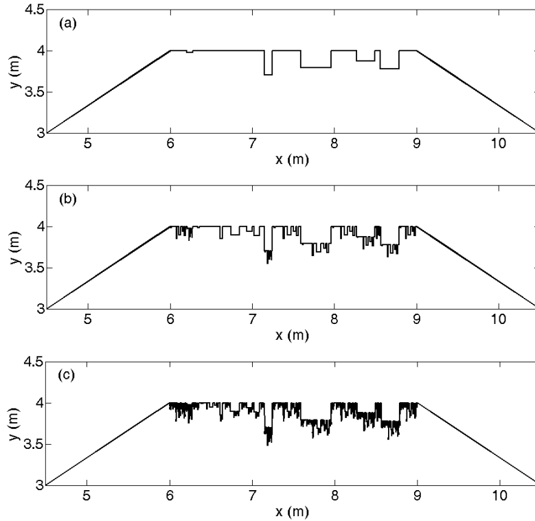
Figure 3. Realisations of roughening the top surface of a trapezoidal berm using rectangular and irregular indentations at orders 1 (a), 2 (b) and 3 (c) (from Ref. [17]).
