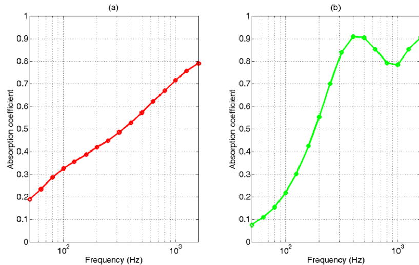
Figure 1. Green-roof substrate (a) and green-wall (b) substrate absorption coefficient upon normal incident sound used in the calculations in Refs. [17], [47] and [159].
