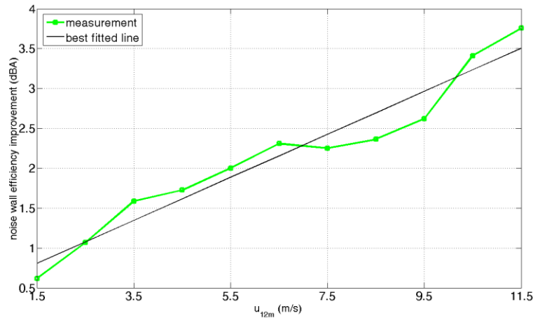
Figure 2. Measured noise wall efficiency improvement resulting from the presence of a tall row of trees at close distance behind a 4-m high motorway noise barrier as a function of downwind wind speed measured at a height of 12 m ( u_{12m} ) (from Ref. [31]).
