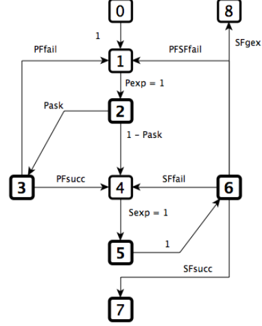
Figure 2. PPP as Markov chain.
