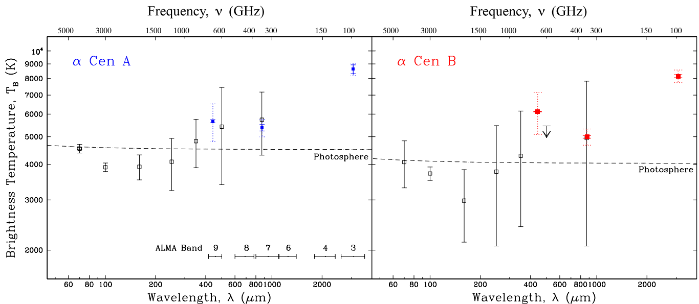
Fig. 3. Far-infrared to submm/mm SEDs of \alpha Cen A ( left ) and \alpha Cen B ( right ), where blue and red symbols identify the respective ALMA measurements. Observational rms-errors are given by solid bars and maximum absolute uncertainties of the ALMA data as dots, where relative values are \leq 15\% for Band 9, \leq 7\% for Band 7, and \leq 5\% for Band 3. With the exception of the point at 70 \mu\text{m} , the data shown by black symbols are based on unresolved single-dish observations (see the text). The extrapolations longward of 45 \mu\text{m} of the PHOENIX model atmospheres (Brott & Hauschildt 2005) are indicated by the dashed lines.
