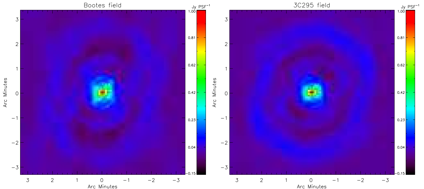
FIG. 2.— Point Spread Functions for the Boötes ( left ) and 3C 295 ( right ) images covering the 54–70 MHz frequency range.
