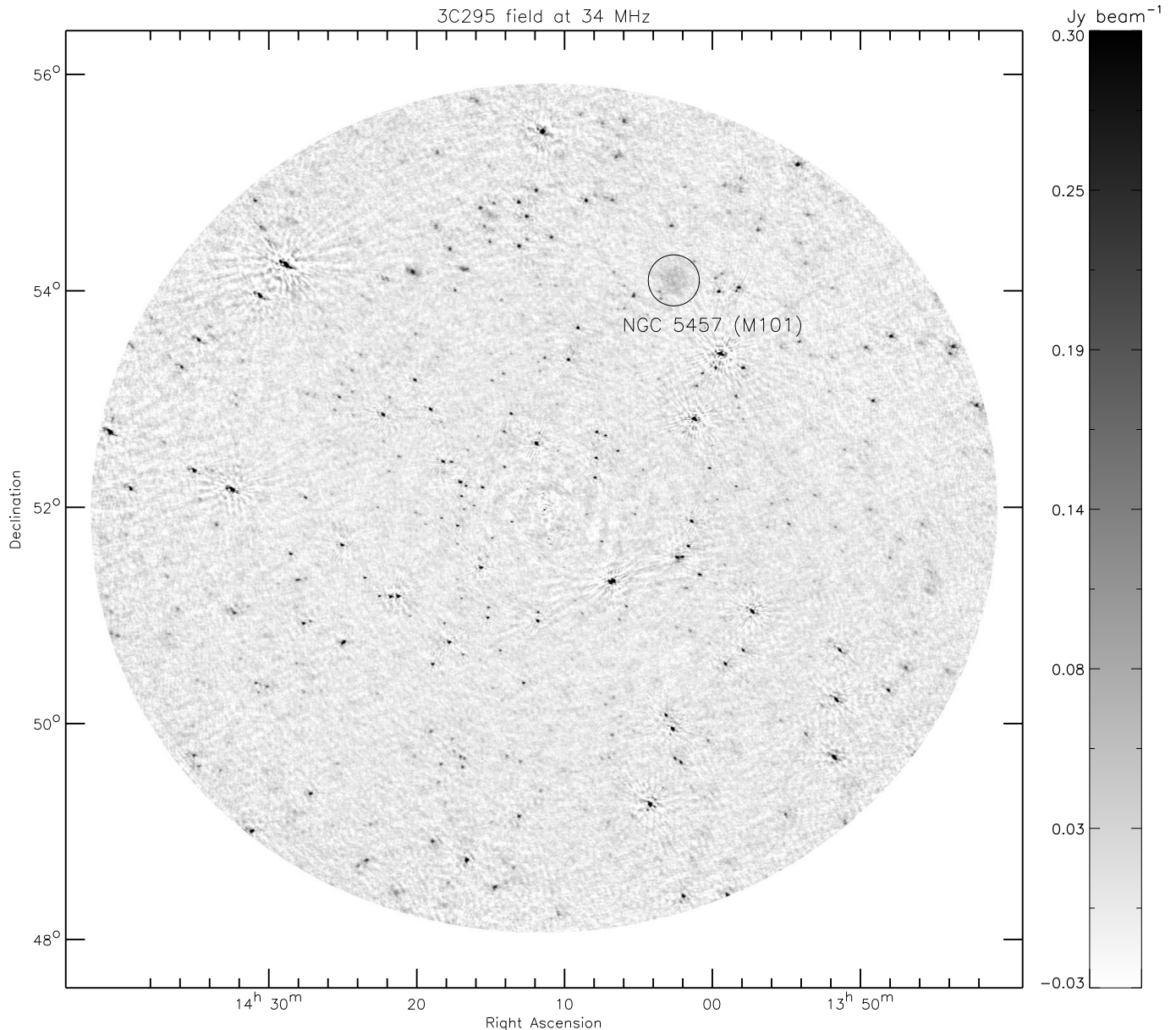
FIG. 7.— Primary beam corrected 3C 295 field 34 MHz image. The image is blanked beyond a primary beam attenuation factor of 0.4. The position of NGC 5457 is indicated.
