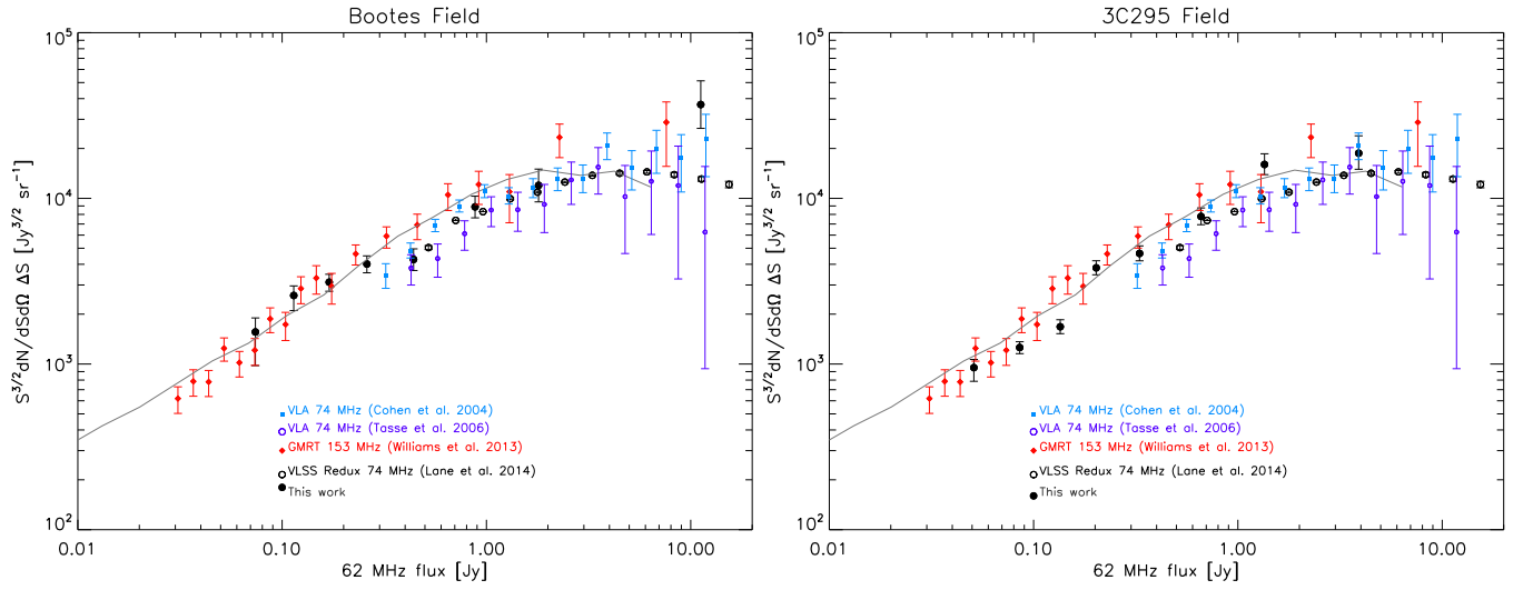
FIG. 20.— Euclidean-normalized differential source counts at 62 MHz for the Boötes and 3C 295 fields. The LOFAR points are indicated by the black symbols. Red diamonds are Boötes field source counts at 153 MHz, scaled to 62 MHz using \alpha = -0.7 . Black open circles, blue squares and purple open circles are 74 MHz differential source counts from Tasse et al. (2006); Cohen et al. (2004); Lane et al. (2014) and the solid grey line displays the counts from the 151 MHz SKADS S^3 -SEX simulation (Wilman et al. 2008). These are all scaled to 62 MHz assuming \alpha = -0.7 .
