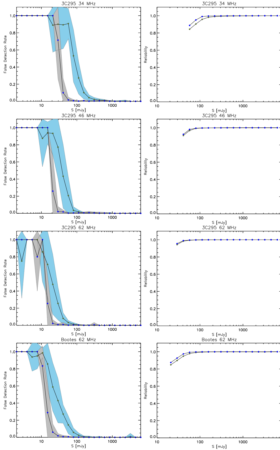
FIG. 12.— False detection rate and reliability. From top to bottom : 3C 295 34, 46 and 62 MHz and Boötes 62 MHz. Left : False detection rate as a function of peak flux density to local signal-to-noise ratio calculated from 25 Monte-Carlo simulations. The solid line shows the mean of all 25 randomly generated fields and the shaded areas show the 1\sigma uncertainty. The blue shaded areas and olive points include source smearing in the MC simulations (see main text of Sect. 3.4). The grey shaded areas and blue points do not include source smearing. Right : Estimated reliability of the catalogue as a function of integrated flux density limit accounting for the varying sensitivity across the field of view. The olive points include source smearing, the blue points do not.
