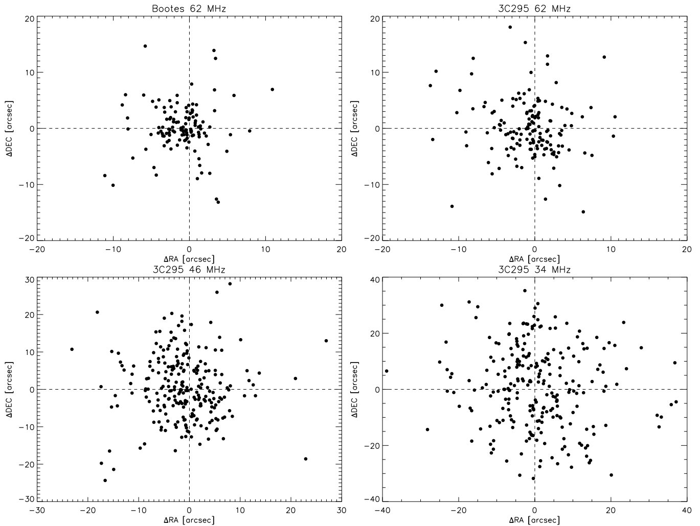
FIG. 9.— The position offsets between the LOFAR LBA and the 325 MHz WENSS sources.
