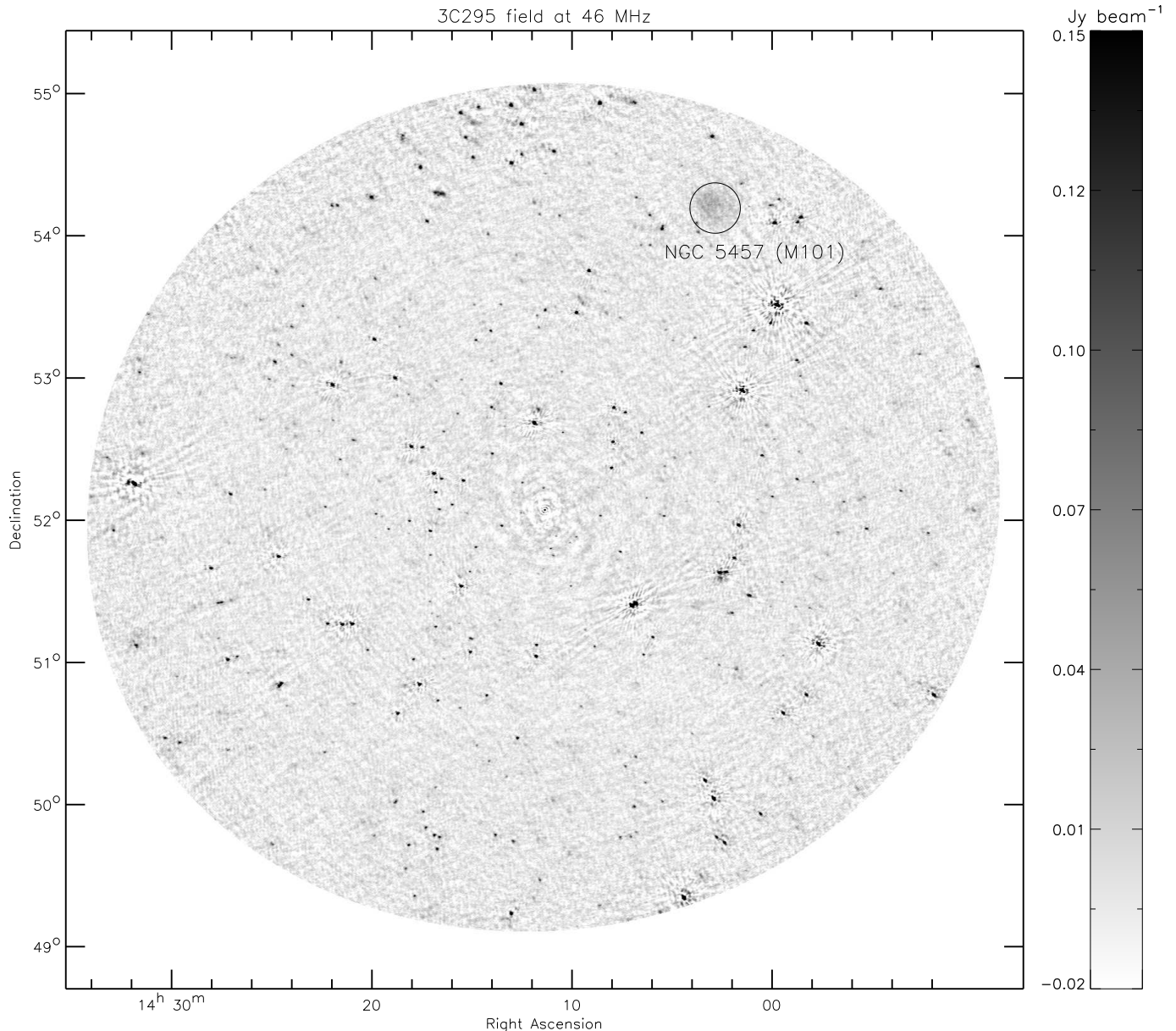
FIG. 6.— Primary beam corrected 3C 295 field 46 MHz image. The image is blanked beyond a primary beam attenuation factor of 0.4. The position of NGC 5457 is indicated.
