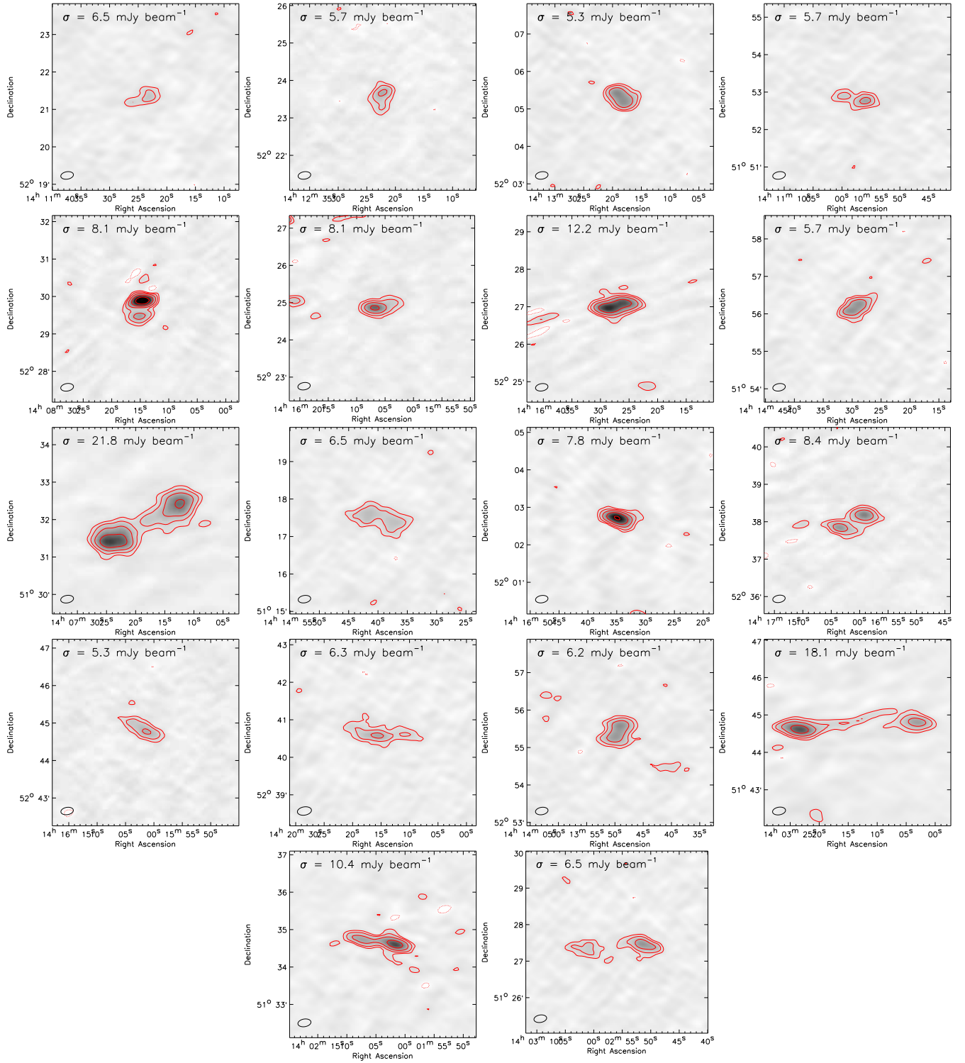
FIG. 17.— Images of resolved sources in the 3C 295 field at 62 MHz. Contour levels are drawn at [1, 2, 4, 8, \dots] \times 3\sigma_{\text{local rms}} , with \sigma_{\text{local rms}} reported in each image. The beam size is shown in the bottom left corner of the images.
