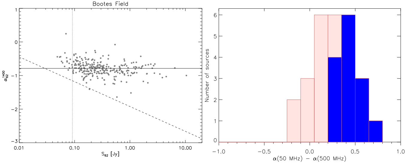
FIG. 15.— Left: Spectral index between 62 and 1400 MHz of sources in the Boötes field plotted against the integrated flux density. The solid line represents the average spectral index of the sources. The vertical dotted line is drawn at 10\sigma_{\text{rms,avg}} and the dashed line indicates the completeness limit due to the NVSS sensitivity. Right: Histogram of spectral curvature between 500 and 50 MHz for bright 34 MHz sources. The spectral curvature was computed by fitting second order polynomials to the flux density measurements. The blue colors represent sources that cannot be properly fitted with power-law spectra and have |a_2| > \sigma_{a_2} , see Sect. 4.2.
