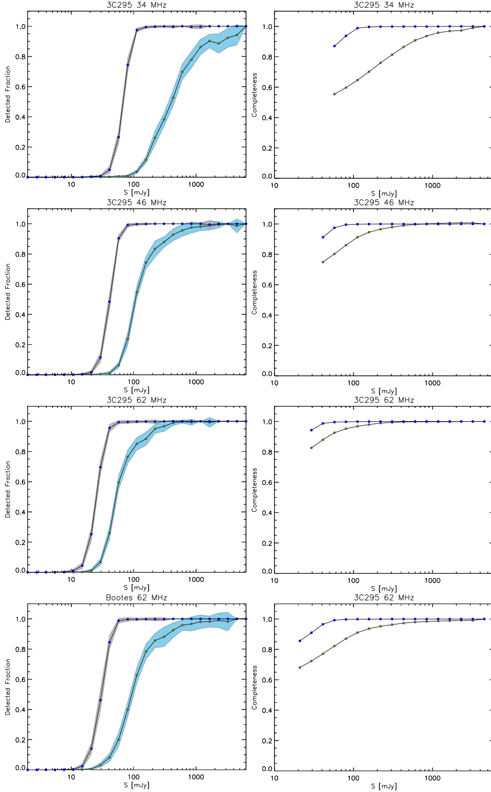
FIG. 11.— Detection fraction and completeness. From top to bottom : 3C 295 34, 46 and 62 MHz and Boötes 62 MHz. Left : Fraction of sources detected as a function of integrated flux density calculated from 25 Monte-Carlo simulations. The solid line shows the mean of all 25 randomly generated fields and the shaded areas show the 1\sigma uncertainty. The blue shaded areas and olive points include source smearing in the MC simulations (see the main text of Sect. 3.4). The grey shaded areas and blue points do not include source smearing. Right : Estimated completeness of the catalogue as a function of integrated flux density limit accounting for the varying sensitivity across the field of view. The olive points include source smearing, the blue points do not.
