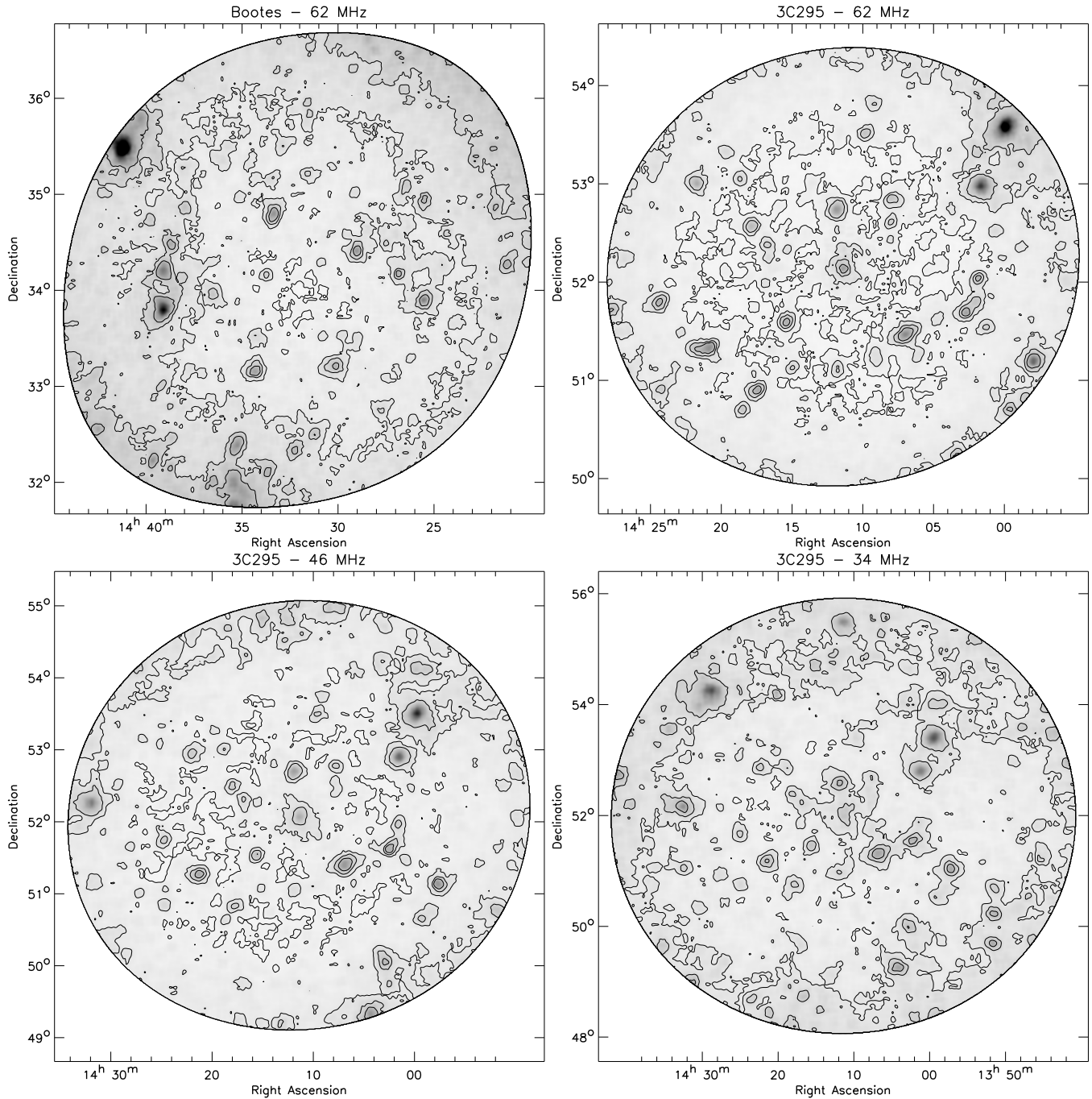
FIG. 3.— Figures showing the local rms noise in the images. A box size of 80 \times 80 pixels was used in computing the local rms noise. The pixel sizes are listed in Table 2. The gray scales display the range from 0.5\sigma_{\text{rms}} to 10\sigma_{\text{rms}} , with the \sigma_{\text{rms}} values taken from Table 2. Contour levels are drawn at (\sqrt{2})^n \times \sigma_{\text{rms}} , with n ranging from -1 to 3 . The local noise variations are correlated with the position of strong sources.
