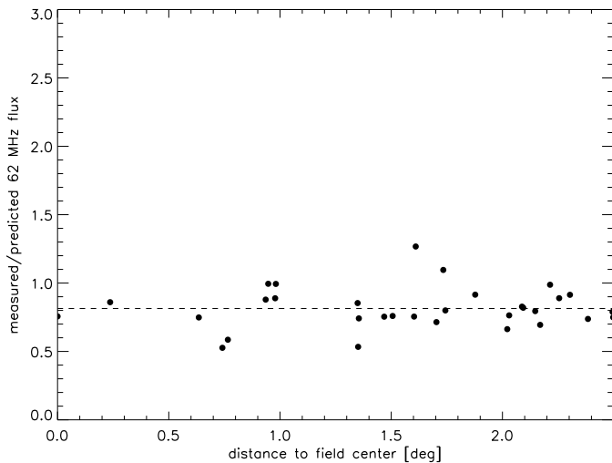
FIG. 10.— Measured flux densities over the predicted flux densities as function of radial distance to the Boötes field center. Dashed line shows the robust mean of the plotted data points.
