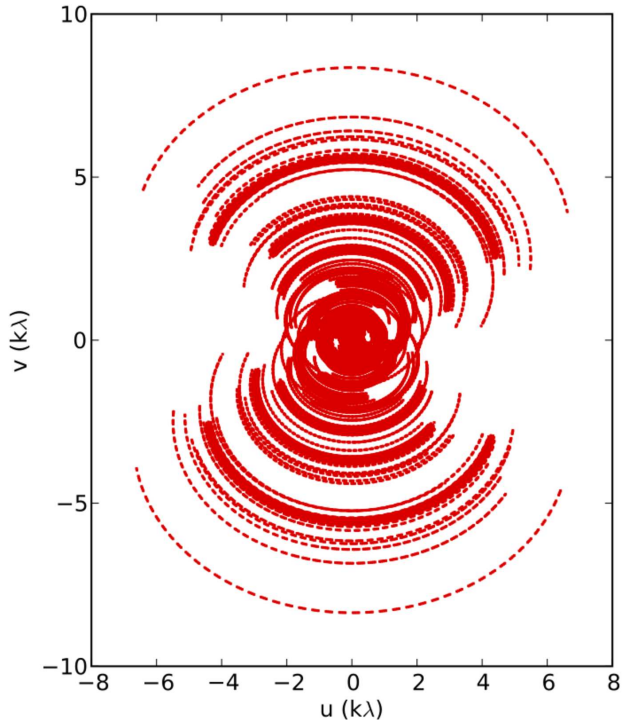
FIG. 1.— UV-coverage of the 3C 295 observations. The relatively large fractional bandwidth fills the uv-plane radially (not shown in the figure).
