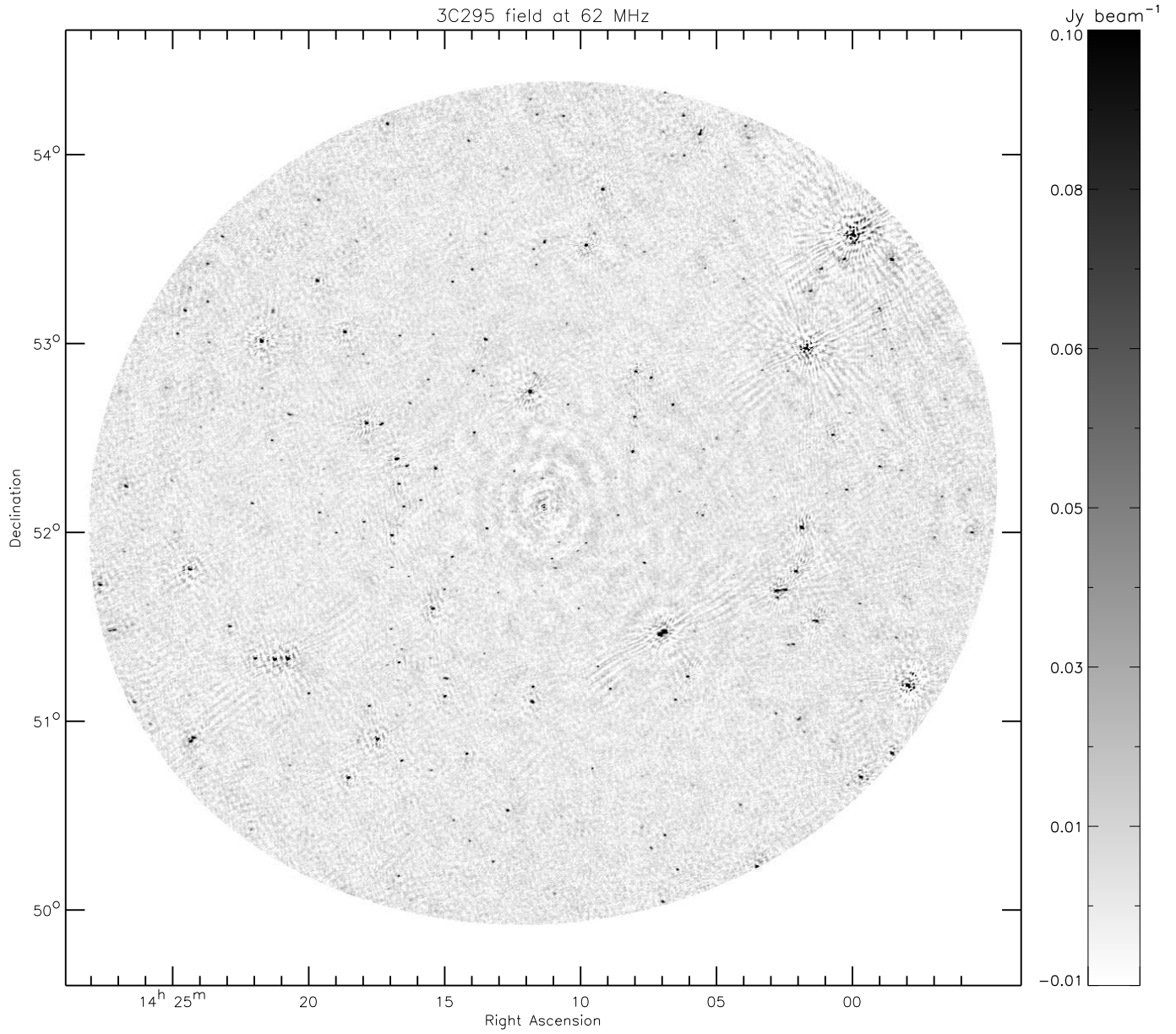
FIG. 5.— Primary beam corrected 3C 295 field 62 MHz image. The image is blanked beyond a primary beam attenuation factor of 0.4.
