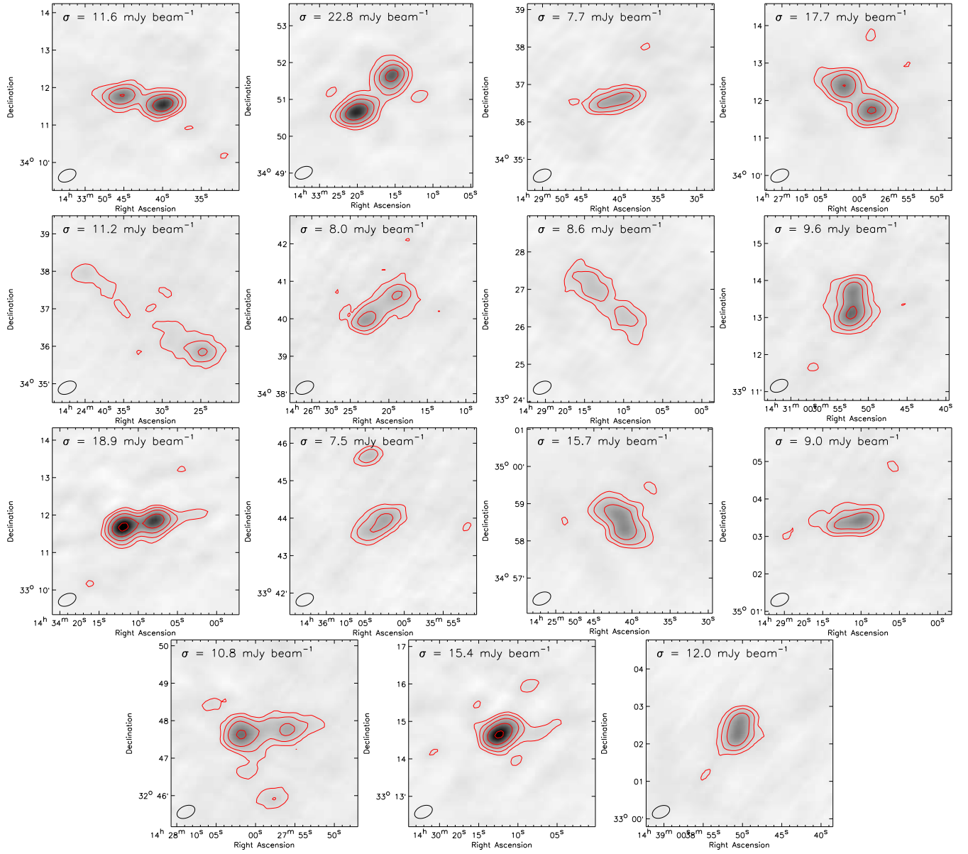
FIG. 16.— Images of resolved sources in the Boötes field at 62 MHz. Contour levels are drawn at [1, 2, 4, 8, \dots] \times 3\sigma_{\text{local rms}} , with \sigma_{\text{local rms}} reported in each image. The beam size is shown in the bottom left corner of the images.
