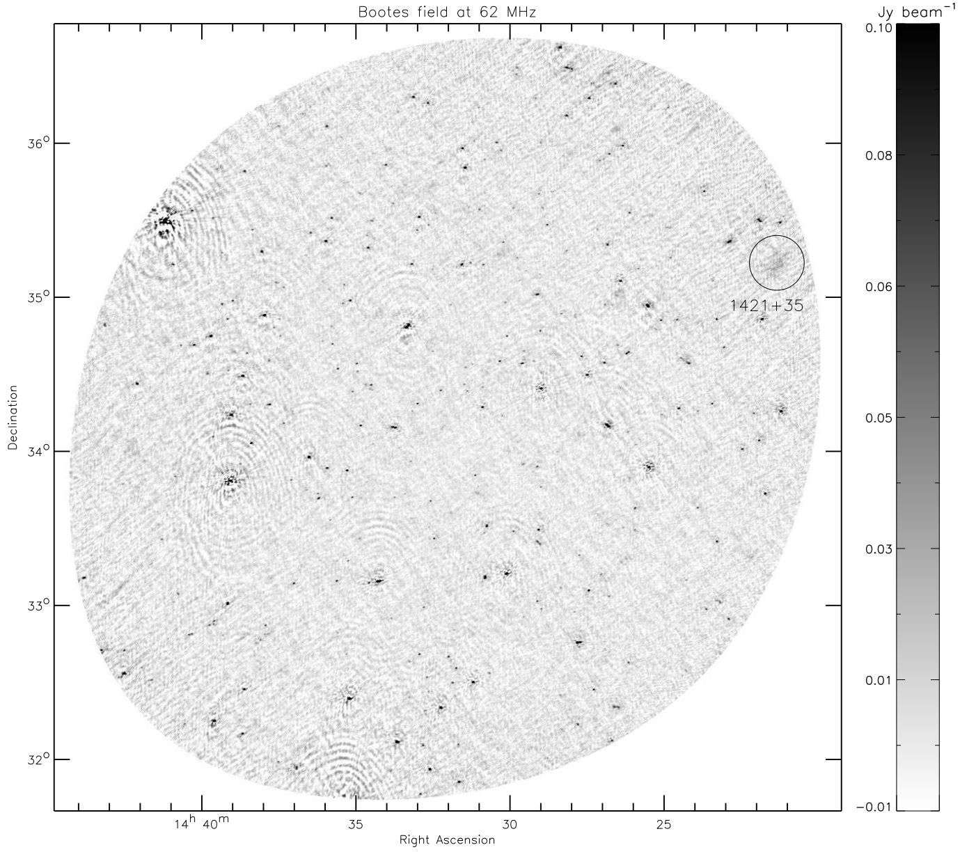
FIG. 4.— Primary beam corrected Boötes field 62 MHz image. The image is blanked beyond a primary beam attenuation factor of 0.4. The position of the diffuse source 1421+35 is indicated.
