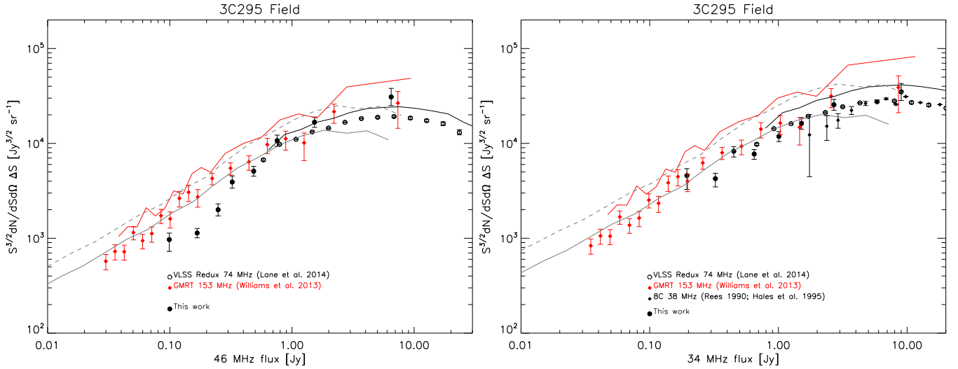
FIG. 14.— Euclidean-normalized differential source counts at 46 ( left ) and 34 MHz ( right ) for the 3C 295 field. The LOFAR points are indicated by the black circles. The red diamonds are Boötes field source counts at 153 MHz and the black open circles show the VLSSr counts at 74 MHz (Lane et al. 2014), both scaled with \alpha = -0.5 . Red and black solid lines show the same source counts but scaled with \alpha = -0.7 . The solid and dashed grey lines displays the counts from the 151 MHz SKADS S^3 -SEX simulation (Wilman et al. 2008) scaled with \alpha = -0.5 and \alpha = -0.7 , respectively. For the 34 MHz panel we have also plotted the 8C source counts at 38 MHz with black diamonds. The 8C source counts are complete to a flux level of about 5 Jy. Below a flux density of 5 Jy we have corrected the source counts using the information provided in fig. 7 from Rees (1990).
