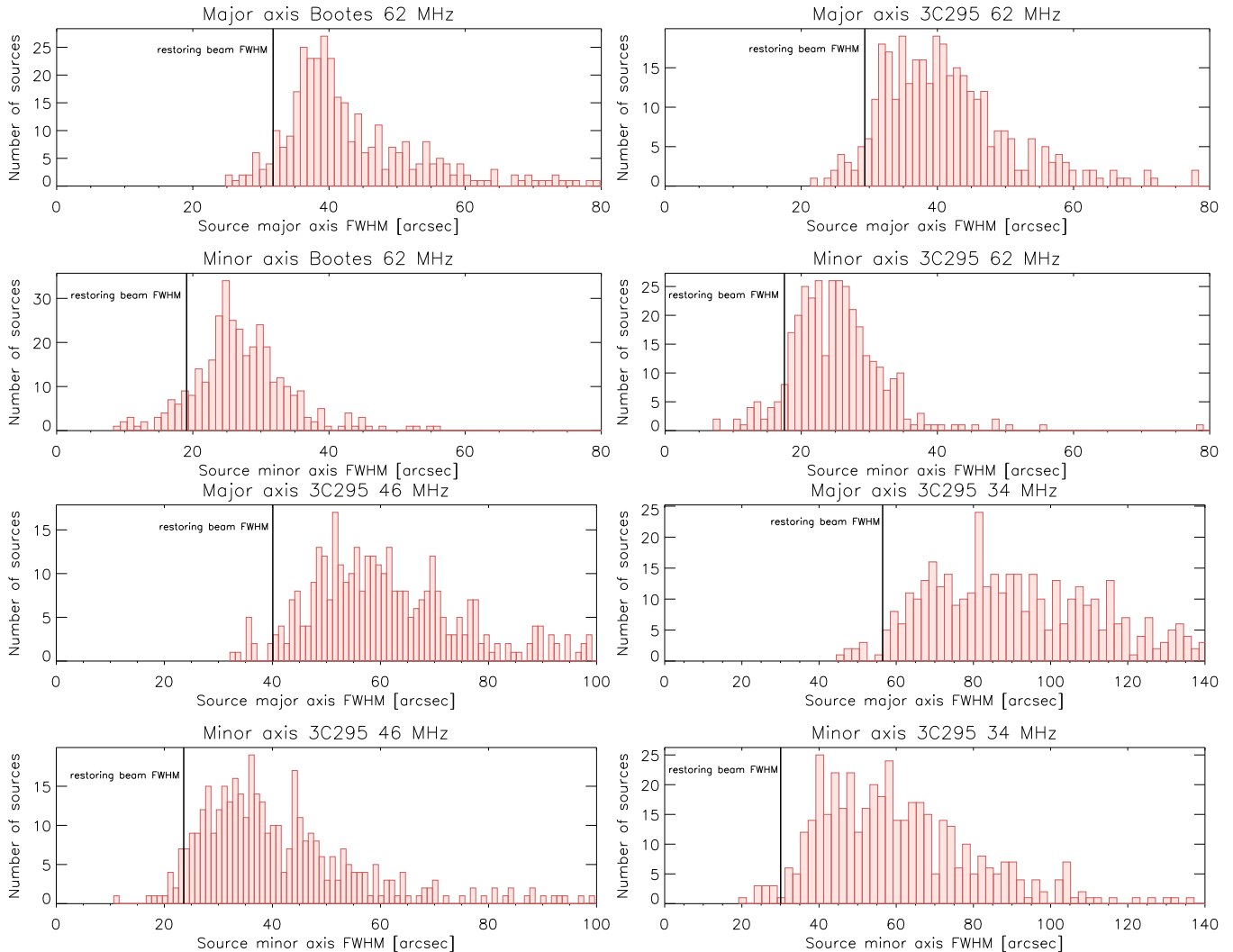
FIG. 8.— Distribution of fitted major and minor axes (full width half maximum) for the Boötes and 3C 295 fields. These values are not deconvolved by the beam. Solid black line indicates the fitted restoring beam based on the uv coordinates. Uncorrected ionospheric phase variations causes “smearing” of sources and decreases the effective resolution. This effect increases towards lower frequencies.
