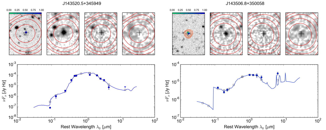
FIG. 18.— Top panels: postage stamps showing NDWFS I-band, IRAC 4.5 micron, IRAC 8.0 micron and MIPS 24 micron images. GMRT 153 MHz (red) and FIRST 1.4 GHz (orange, when available) contours are overlaid. Radio contour levels are drawn at [1, 2, 4, \dots] \times 3\sigma_{\text{rms}} . A black cross indicates the GMRT radio position and the color scale at the top of the I-band image shows the probability that the I-band source, marked with a colored point, is the true optical counterpart. Bottom panels: Spectral energy distribution and best fitted LRT model for the optical counterpart(s). The flux measurements were taken from Jannuzi & Dey (1999); Elston et al. (2006); Cool (2007); Ashby et al. (2009); Morrissey et al. (2007); Jannuzi et al. (2010).
