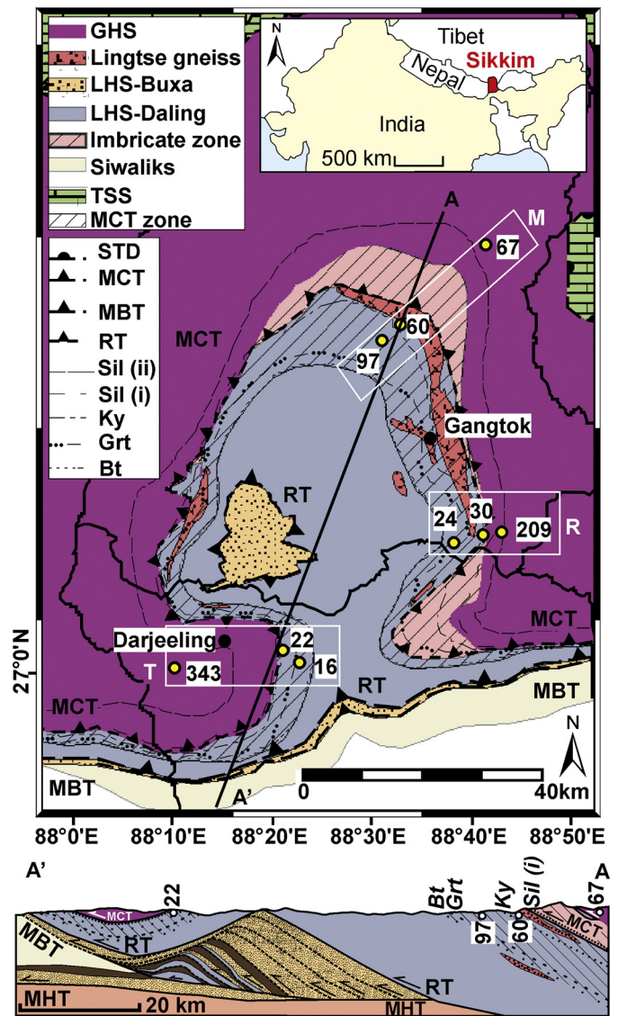
Fig. 1. Geological map and cross section (to scale) of the Sikkim Himalaya, adapted from Mottram et al. (2014). Sample locations are shown for the three boxed transects (T = Takdah, M = Mangan and R = Rongli). Abbreviations: STD = South Tibetan Detachment, MCT = Main Central Thrust, RT = Ramgarh Thrust, MBT = Main Boundary Thrust, MHT = Main Himalayan Thrust, Sil (ii) = sillimanite (no muscovite), Sil (i) = fibrolite, Ky = kyanite, Grt = garnet, Bt = biotite, GHS = Greater Himalayan Sequence, LHS = Lesser Himalayan Sequence, B = Buxa, D = Daling, IZ = Imbricate Zone (Mottram et al., 2014), SW = Siwaliks, TSS = Tethyan Sedimentary Sequence. Lesser Himalayan Duplex schematic representation of Bhattacharyya and Mitra (2009). The zone of deformation associated with the Main Central Thrust is shown as a hatched area.
