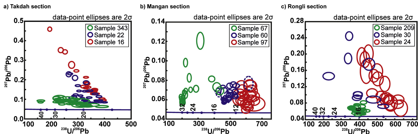
Fig. 6. Summary of all monazite U–Th–Pb data plotted in Tera–Wasserburg plots for the three sections from the Sikkim Himalaya (locations in Fig. 1). In each plot the structurally highest GHS sample is shown in green, the upper LHS sample in blue and the structurally lowest LHS sample in red. Detailed plots for each transect can be found in Fig. 7 for the Takdah transect, and in the supplementary material S4.3 for the Mangan and Rongli sections. (For interpretation of the references to colour in this figure legend, the reader is referred to the web version of this article.)
