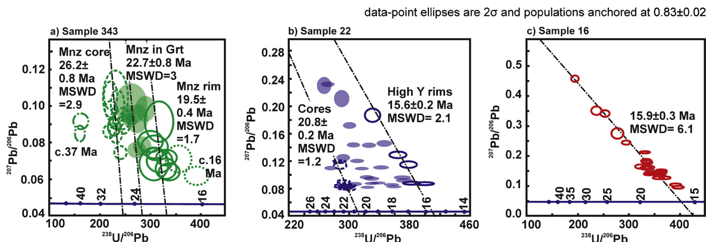
Fig. 7. Detailed Tera–Wasserburg plots for the Takdah transect. The GHS sample 343 in green, upper LHS sample 22 shown in blue and lower LHS sample 16 is shown in red. All data uncorrected for common Pb; intercepts are anchored at the common-Pb value of 0.83 \pm 0.02 (Stacey and Kramers, 1975). (For interpretation of the references to colour in this figure legend, the reader is referred to the web version of this article.)
