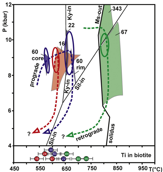
Fig. 5. Summary of pressure–temperature conditions for all samples. The lowest grade LHS samples are represented by the red field and arrow (sample 16 and representative of samples 24 and 97). The upper LHS samples have a more prolonged prograde and peak history as demonstrated by the blue fields and arrow for samples 22 and 60 (representative of sample 30). The peak metamorphic fields for the GHS samples are shown in green and by the green arrow (for samples 67 and 343 and representative of sample 209). Ti in biotite measurements are shown in the lower box. As the thermometer is calibrated for pressures of \sim 4\text{--}6 kbar (Henry et al., 2005), somewhat lower than the ambient pressure conditions, a conservative error of \pm 50^\circ\text{C} has been applied to each measurement. (For interpretation of the references to colour in this figure legend, the reader is referred to the web version of this article.)
