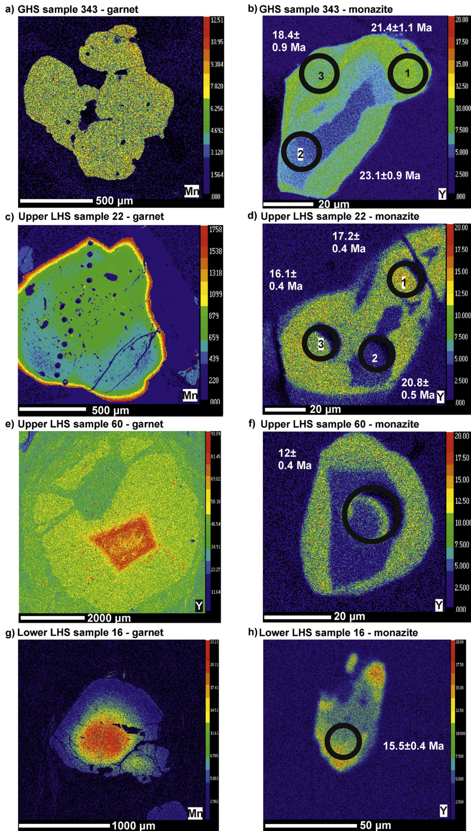
Fig. 2. Garnet (a, c, e, g) and monazite (b, d, f, h) X-ray maps demonstrating zoning in major (Mn) and trace (Y) elements. Monazite maps show ^{238}\text{U}/^{206}\text{Pb} ages with 2\sigma errors.
