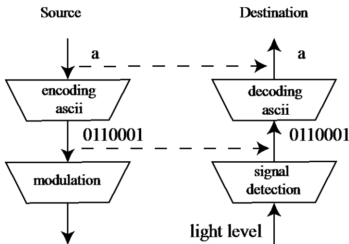
Figure 2. A communication system with two levels
