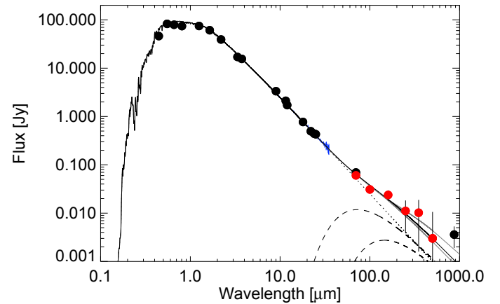
Fig. 6. SED of HIP 92043. Optical, near infrared and LABOCA 870 \mu\text{m} point in black, the Spitzer IRS spectrum in blue, Herschel fluxes in red. Uncertainties are 1\text{-}\sigma and may be smaller than the data point. The stellar photosphere is denoted by a dotted line. The solid black line denotes the sum of the stellar photosphere and a pair of black bodies (70 and 30 K, dashed lines). The solid grey lines denote the effect on the SED of altering the cold component temperature by \pm 10 K.
