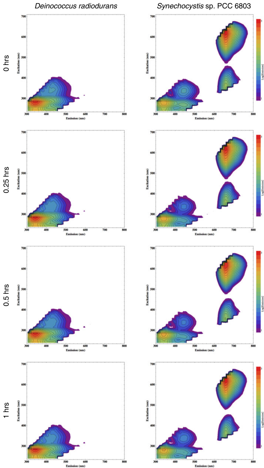
Fig. 3. The complete EEM dataset acquired on the fluorescence response of the two model organisms after increasing UV irradiation. Emission intensity is in arbitrary units and colour-coded on a log-10 scale as indicated. The total UV doses used are calibrated to the equivalent number of hours of exposure on the Martian surface, calculated for equatorial noontime conditions (Patel et al. 2002): 0.25, 0.5, 1, 2, 4, 8 and a maximum of 32 h Mars-equivalent exposure for Deinococcus and 64 h for Synechocystis . Minimal degradation of fluorescence signal is observed for Deinococcus , but the cyanobacterium exhibits noticeable diminishment of photosystem fluorescence (peaking at an excitation–emission wavelength pairing of about 615–660 nm) and a stark increase in the fluorescent feature at an ex–em pairing of about 340–440 nm.
