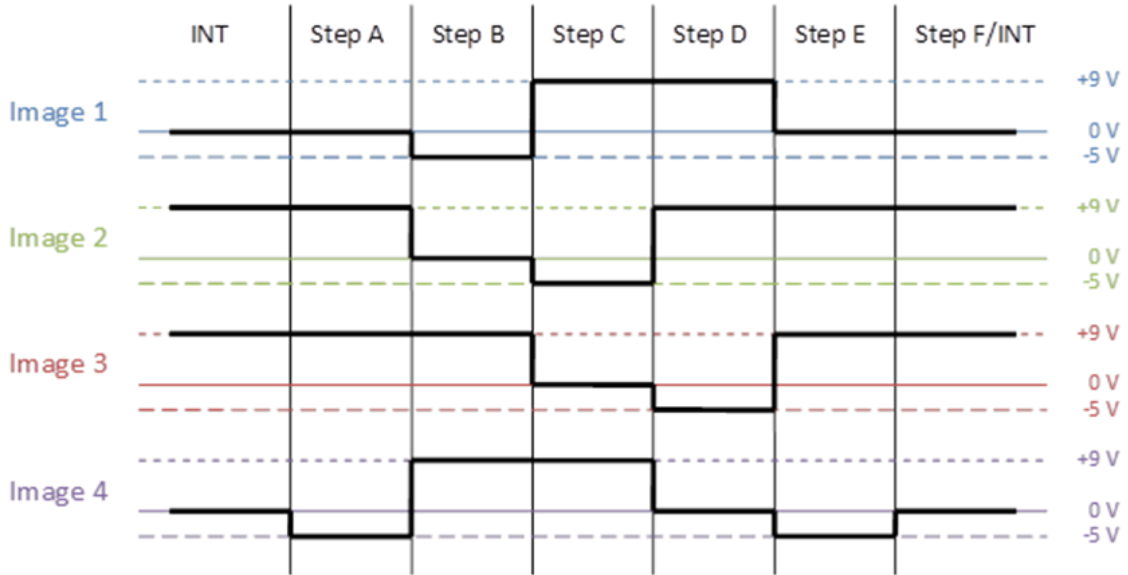
Figure 1. Example of a multiple (three) level parallel clocking scheme.
