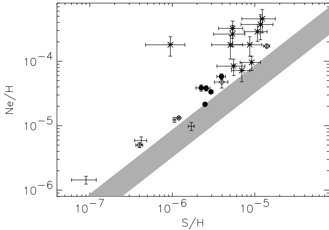
FIG. 2.—Ne/H vs. S/H abundance. Our BCDs are indicated by filled circles if \text{H}\alpha is detected and by diamonds if it is not detected. The sources that are shown by only the error bars are those that have a nondetection of [\text{Ne II}] or [\text{S III}] (see the note to Table 4). The starburst galaxies from Verma et al. (2003) are marked with stars. We use the gray band to indicate the locus on the plot where the ratio of Ne/S would be consistent with the different solar values for neon and sulfur abundances.
