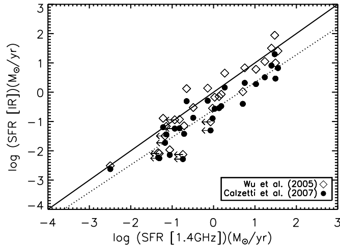
FIG. 4.—Plot of the SFR based on the 24\ \mu\text{m} luminosity as a function of the corresponding SFR estimated from the 1.4 GHz radio continuum emission for each galaxy in our sample. The open diamonds indicate the SFRs calculated using the 24\ \mu\text{m} fluxes following Wu et al. (2005; eq. [1]); the filled circles indicate those using eq. (2) from Calzetti et al. (2007). The solid line is the 1 : 1 proportionality line. The dotted line is a fit to the filled circles.
