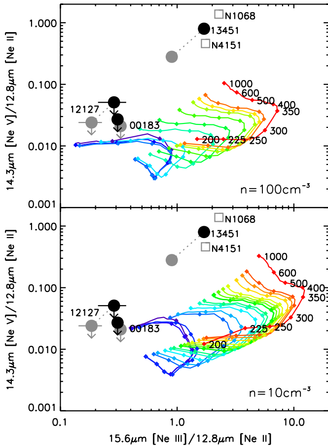
Figure 9. Mid-infrared diagnostic diagram for the line ratio 15.56 \mu\text{m} [Ne III] / 12.81 \mu\text{m} [Ne II] versus 14.32 \mu\text{m} [Ne V] / 12.81 \mu\text{m} [Ne II]. Plotted are predicted line ratios as computed by MAPPINGS version IIIq (Allen et al. 2008) for combined precursor+shock models at solar metallicity at a gas density n = 100 \text{ cm}^{-3} (upper panel) and n = 10 \text{ cm}^{-3} (lower panel). Different colors (ranging from purple to red) denote different magnetic field strengths, ranging from 10^{-3} to 100 \mu\text{G} . Shock velocities range from 200 to 1000 \text{ km s}^{-1} and are labeled along the red curve. Overlaid are the positions of IRAS F00183–7111, IRAS 12127+1412NE and IRAS 13451+1232 for the integrated fluxes (gray disks) and for just the blueshifted component (black disks). Gray squares mark the positions of the nuclear spectra of the classical AGNs NGC 1068 and NGC 4151 (Sturm et al. 2002).
