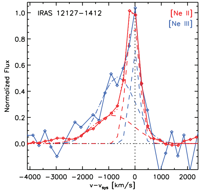
Figure 6. Comparison of the galaxy-integrated line profiles of 12.81\ \mu\text{m} [Ne II] (red) and 15.56\ \mu\text{m} [Ne III] (blue) for IRAS 12127-1412NE at a spectral resolution of R = 600 . Overplotted are two-component Gauss fits to the line profiles. The individual components are shown as dashed lines, their sums as dotted lines.
