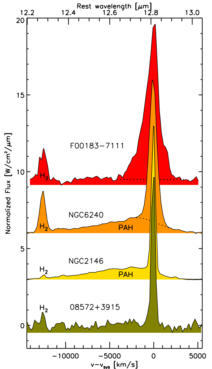
Figure 4. Comparison of the continuum-subtracted spectral structure around the 12.81 \mu\text{m} [Ne II] line for four galactic nuclei, at a spectral resolution R = 600 . The spectral features included are the H 2 S(2) line at 12.28 \mu\text{m} , the 12.7 \mu\text{m} PAH emission feature (extending from -13,500 to +3,500 \text{ km/s} ) and the [Ne II] line. The latter is clearly broadened in the spectra of IRAS F00183–7111 and NGC 6240. Note that the 12.7 \mu\text{m} PAH emission feature appears to be absent in the spectra of IRAS F00183–7111 and IRAS 08572+3915NW.
