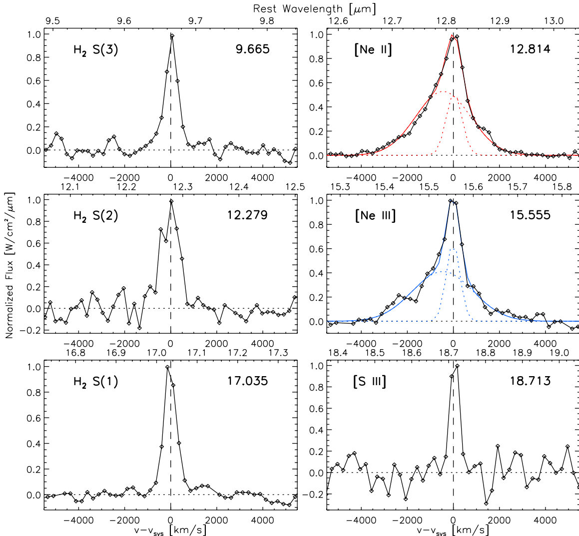
Figure 3. Comparison of the emission line profiles for the six detected emission lines in the spectrum of IRAS F00183–7111. The left column shows the S(1), S(2) and S(3) pure rotational H 2 lines, the right panel the [Ne II], [Ne III] and [S III] lines. All six lines have been observed at the same spectral resolution R = 600 . The [Ne II] and [Ne III] line profiles are clearly asymmetric and broadened beyond the instrumental spectral profile (FWHM = 500 km s -1 ). Their profiles are fit by two Gaussian components (red and blue dotted lines, respectively), the sum of which is shown as a red or blue continuous line.
