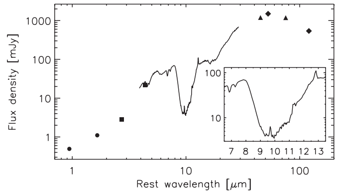
Figure 2. Near-to-far-infrared spectral energy distribution of IRAS F00183–7111. The 4–29 \mu\text{m} Spitzer -IRS low-resolution spectrum (Spoon et al. 2004) is shown as a continuous line. Photometric points are labeled with the following symbols: circles: ESO-NTT J & K (Rigopoulou et al. 1999), squares: IRAC 3.6 & 5.8 \mu\text{m} , triangles: IRAS 60 & 100 \mu\text{m} , diamonds: MIPS 70 & 160 \mu\text{m} . Error bars on the photometric points are too small to be visible. Inset: detailed view of the spectral range around the 9.7 \mu\text{m} silicate absorption profile. Note the emission lines of \text{H}_2 \text{ S}(3) at 9.66 \mu\text{m} and [\text{Ne II}] at 12.81 \mu\text{m} .
