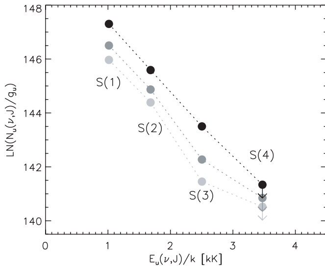
Figure 10. Excitation diagram for warm molecular hydrogen in IRAS F00183–7111 based on the line fluxes for the pure-rotational transitions S(1)–S(4). Different shades of gray are used to distinguish different levels of dereddening: black: A_V = 25 , dark gray: A_V = 10 , light gray: A_V = 0 . Error bars are too small to be visible.
