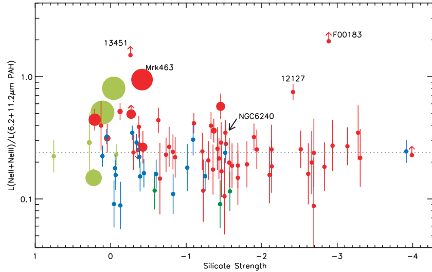
Figure 8. Ratio of the combined [Ne II]+[Ne III] luminosity and the combined PAH(6.2 \mu\text{m} )+PAH(11.2 \mu\text{m} ) luminosity as a function of silicate strength (Spoon et al. 2007). The symbol size scales linearly with the [Ne V]/[Ne II] ratio above a threshold ratio of 0.4. The largest symbol corresponds to a [Ne V]/[Ne II] ratio of 2.2. The horizontal dotted line indicates the average neon/PAH ratio for low-excitation ULIRGs. IRAS F00183–7111 is more than a factor 8 above this value, indicating that it is overluminous in its neon lines compared to its PAH emission. The same is true to a lesser extent for the ULIRGs IRAS 12127–1412NE and IRAS 13451+1232. Galaxy types are labeled as follows: ULIRGs: red, starburst galaxies: blue, Seyfert-2 galaxies: dark green, Seyfert-1 galaxies and QSOs: light green.
