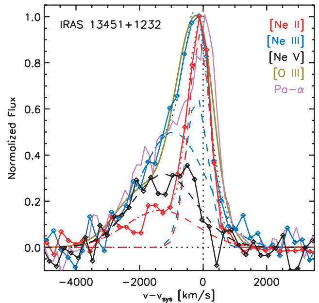
Figure 7. Comparison of the galaxy-integrated line profiles of 12.81\ \mu\text{m} [Ne II] (red), 15.56\ \mu\text{m} [Ne III] (blue) and 14.32\ \mu\text{m} [Ne V] (black) for IRAS 13451+1232 at a spectral resolution of R = 600 . Overplotted are two-component Gauss fits to the neon line profiles. The individual components are shown as dashed lines, their sums as dotted lines. The [Ne V] line has been scaled to match the blue wing of the [Ne III] line profile. Also shown is the sum of the three-component Gauss fit to the 5007\ \text{\AA} [O III] line (green) as presented by Holt et al. (2003), degraded to a resolution of R = 600 , and the Pa \alpha profile (purple) obtained by Veilleux et al. (1997) at R = 650 .
