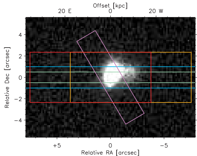
Figure 1. K -band image of IRAS F00183–7111 replotted from Rigopoulou et al. (1999). North is up, east is to the left. Overlaid on the image are the various slits used to obtain spectra of the emission line features discussed in the paper. In red and orange is the Spitzer -IRS SH slit in the two nodding positions; in blue is the slit used by Heckman et al. (1990), in green the slit used by Dannerbauer et al. (2005), and in purple the slit used by Buchanan et al. (2006). (A color version of this figure is available in the online journal.)
