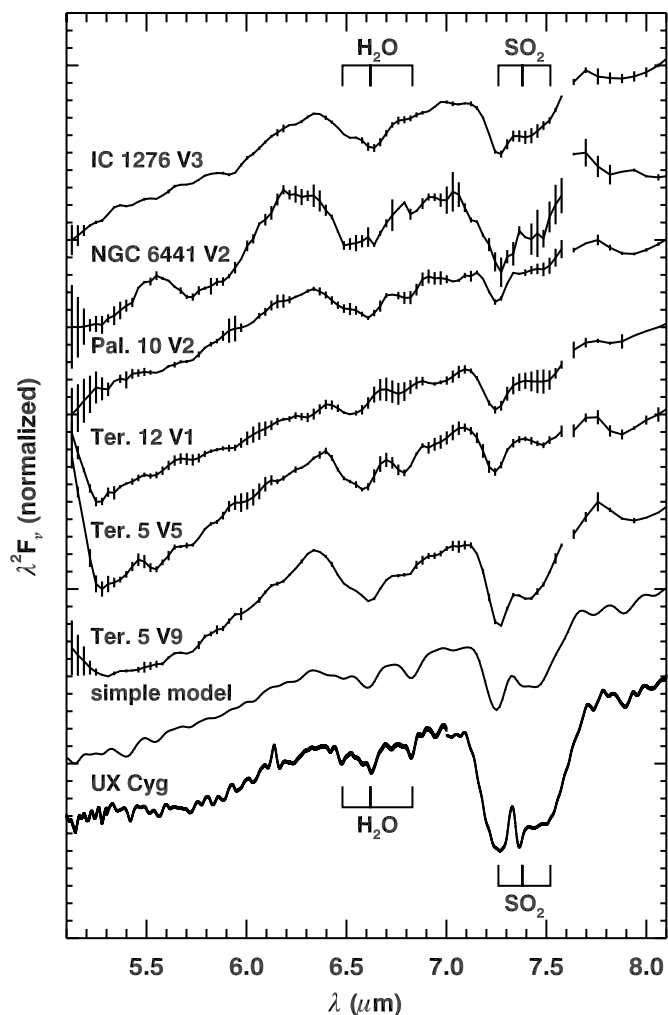
Figure 18. Six IRS spectra showing \text{SO}_2 absorption bands at 7.3\text{--}7.5\ \mu\text{m} , along with a simple model and a comparison spectrum of a Galactic AGB star, UX Cyg, obtained with the SWS on ISO . The spectra are plotted in Rayleigh–Jeans units ( \lambda^2 F_\nu or \lambda^4 F_\lambda ) so that the Rayleigh–Jeans tail of the blackbody function would be a horizontal line. All of the spectra also show absorption from water vapor at 6.4\text{--}6.8\ \mu\text{m} . The simple model includes absorption from only \text{H}_2\text{O} and \text{SO}_2 .
