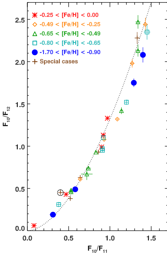
Figure 12. Continuum-subtracted flux ratios of the globular sample compared to the silicate dust sequence (dashed line). The symbols are color-coded as in Figure 10. The circled brown cross in the lower left is the carbon star Lyngå 7 V1. The four points to the right of the silicate dust sequence (with 1.3 < F_{10}/F_{12} < 1.8 ) are, from top to bottom, NGC 6712 V7, NGC 6838 V1, NGC 6356 V5, and NGC 6760 V4, and their deviation from the silicate dust sequence may result from as-yet-unidentified impurities in the dust.
