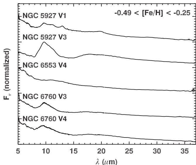
Figure 3. IRS spectra of the five sources in our sample with metallicities ( [Fe/H] ) between -0.25 and -0.49 .
