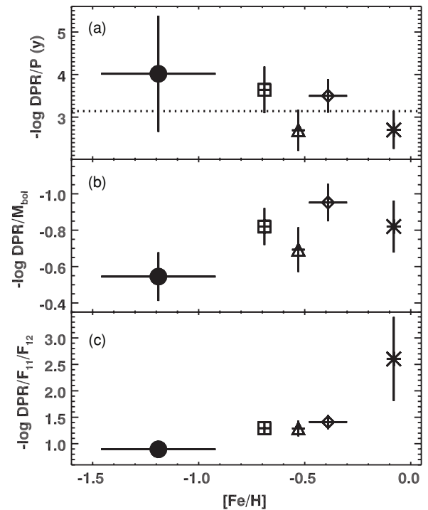
Figure 14. Slopes from Figure 13 plotted as a function of metallicity, with vertical error bars based on the uncertainty in the mean (standard deviation divided by the square root of the sample size). These plots show more clearly how the dust-production rate depends on bolometric magnitude and position along the silicate dust sequence ( F_{11}/F_{12} ), but not on pulsation period (as indicated by the horizontal dotted line in panel (a)). Symbol shapes are the same as defined for Figures 10, 12, and 13.
