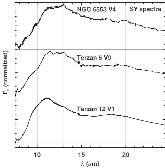
Figure 16. Dust excess, after fitting and subtracting a stellar continuum, from the three spectra classified as “SY” due to their unusual 11–12 \mu\text{m} emission features. The vertical lines appear at wavelengths of 10, 11, 12, 13, and 20 \mu\text{m} .
