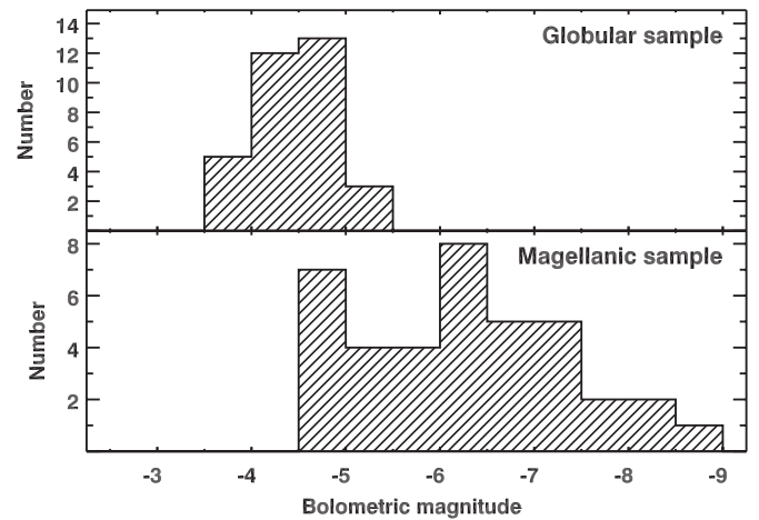
Figure 11. Comparison of the bolometric magnitudes of our globular sample of AGB stars and the Magellanic sample of Sloan et al. (2008). The histogram of the globular sample excludes the four Cepheid variables (all with bolometric magnitudes between -1.6 and -2.7 ) and the four sources whose cluster membership is in doubt.
