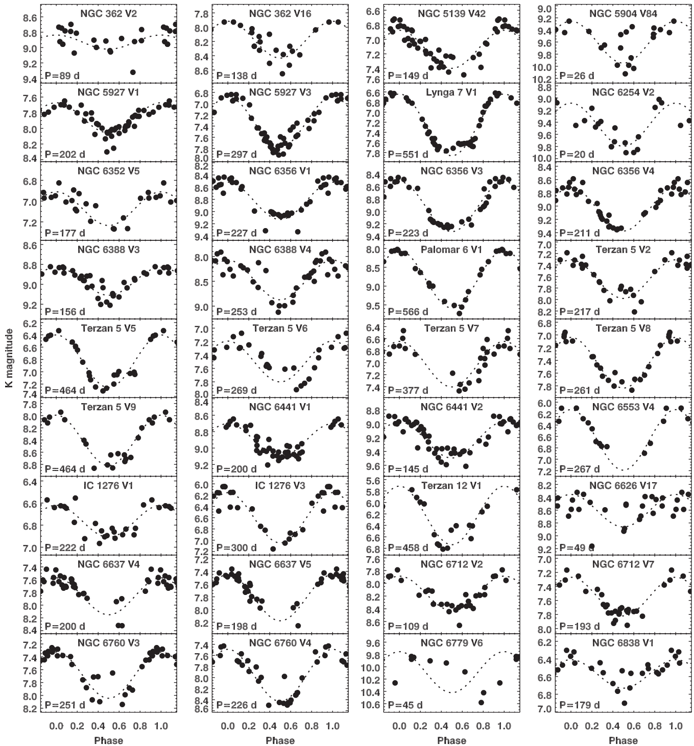
Figure 1. Light curves in the K band for the sources in our sample observed with SIRIUS at the IRSF 1.4 m reflector. Table 2 presents the fitted periods, mean magnitudes, K -band amplitude, and zero-phase dates.
