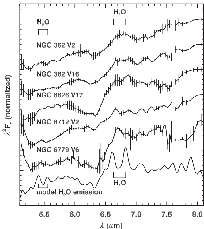
Figure 20. Five IRS spectra showing an apparent absorption feature at \sim 6.35 \mu\text{m} . The spectra are in Rayleigh–Jeans units, as in Figures 18 and 19. The model shows water vapor in emission, and it matches the structure seen in the data reasonably well.
