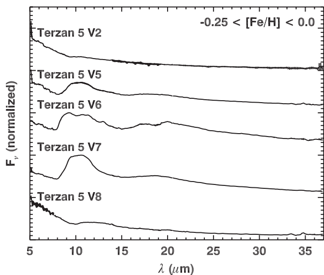
Figure 2. IRS spectra of the five sources in our sample with metallicities ( [Fe/H] ) between 0.0 and -0.25 . The error bars are generally smaller than the width of the plotted spectra.
