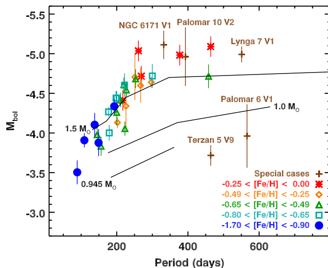
Figure 10. Bolometric magnitudes and pulsation periods of the globular sample, compared to models of AGB stars at 0.945, 1.0, and 1.5 M_{\odot} (black lines; Vassiliadis & Wood 1993). The symbols are color-coded to run from the most metal-rich globular cluster (red) to the most metal-poor (blue), with special cases in brown.
