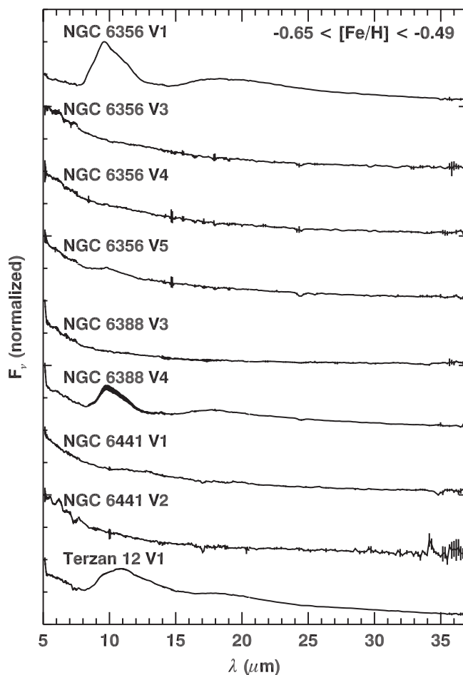
Figure 4. IRS spectra of the nine sources in our sample with metallicities ( [Fe/H] ) between -0.49 and -0.65 .
