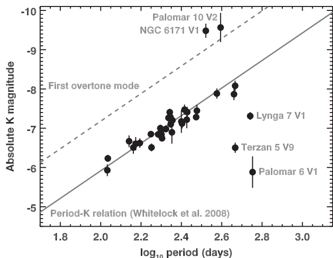
Figure 9. Periods and absolute K magnitudes of the variables in our globular cluster sample (excluding Cepheids). Absolute magnitudes are determined from the distance moduli for the clusters reported in Table 1. The solid line is the nominal period– K relation defined by Whitlock et al. (2008). The dashed line represents the shift in the relation expected for stars pulsating in the first overtone mode. Sources which do not follow the period– K relation are labeled (see Section 3.4).
