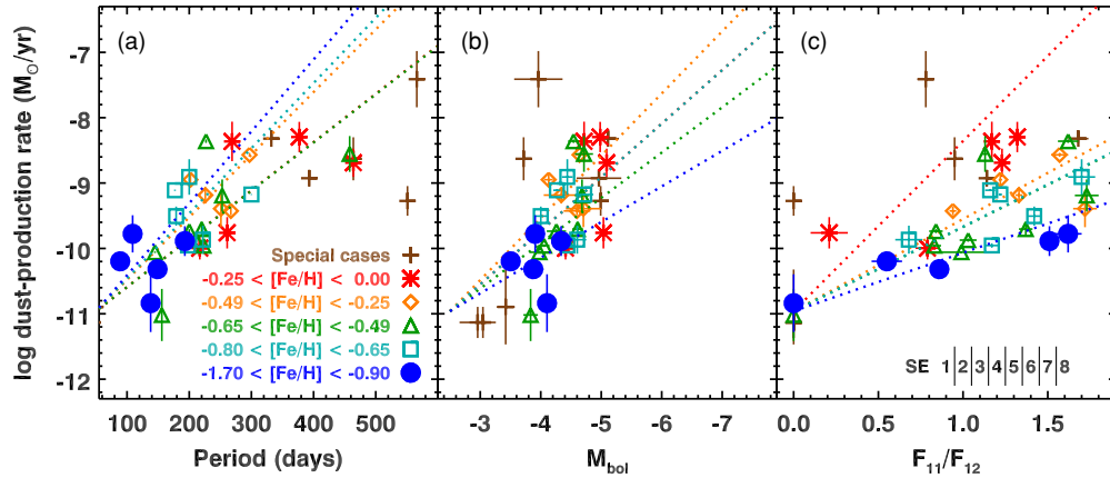
Figure 13. Log of the dust-production rate (DPR) for each of the stars in our sample as a function of pulsation period (panel (a)), bolometric magnitude (panel (b)), and corrected flux ratio F_{11}/F_{12} (panel (c)). The overall MLR is the product of the DPR and the gas-to-dust ratio, which in Table 4 is assumed to be 200 (a difference of 2.30 in log space). The corrected flux ratio in panel (c) locates the position of a source along the silicate dust sequence (Figure 12) and measures the relative contributions from amorphous alumina (low F_{11}/F_{12} ) and amorphous silicates (high F_{11}/F_{12} ). The dotted lines give the mean slope of each metallicity group, assuming a common y-intercept, as explained in the text.
