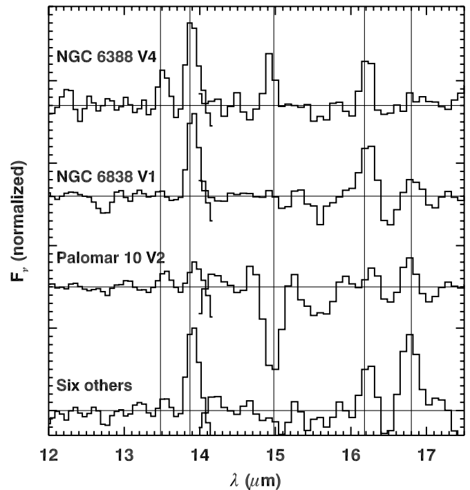
Figure 17. Carbon dioxide emission bands in the spectra of three individual sources and the coaddition of six more. A spline has been fitted and removed from each spectrum, and the residual normalized to the maximum emission or absorption. The horizontal lines mark zero excess flux in each spectrum, and the vertical lines are at wavelengths of 13.48, 13.87, 14.98, 16.18, and 16.80 \mu\text{m} . The coadded spectrum at the bottom includes IC 1276 V1, NGC 5139 V42, NGC 5927 V1, NGC 6171 V1, NGC 6637 V4, and NGC 6760 V3.
