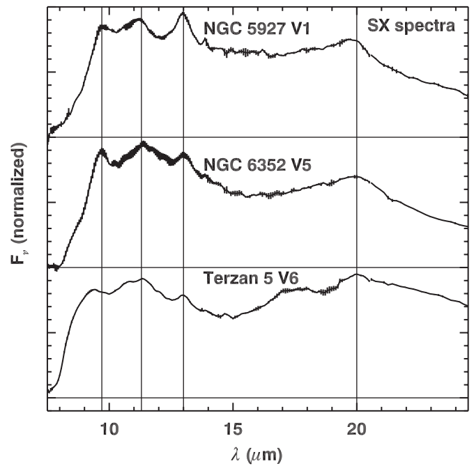
Figure 15. Three spectra classified as “SX” due to the likely presence of crystalline SE at 10 and 11 \mu\text{m} . These spectra are plotted after a stellar continuum has been fitted from 6.8 to 7.4 \mu\text{m} and removed. All three show features at each of the wavelengths marked by vertical lines: 9.7 , 11.3 , 13 , and 20 \mu\text{m} . Terzan 5 V6, with the “ 9.7 ” \mu\text{m} feature shifted to 9.3 \mu\text{m} and a clear contribution from silicates at 18 \mu\text{m} feature, may be affected by some self-absorption in the 10 \mu\text{m} silicate feature.
