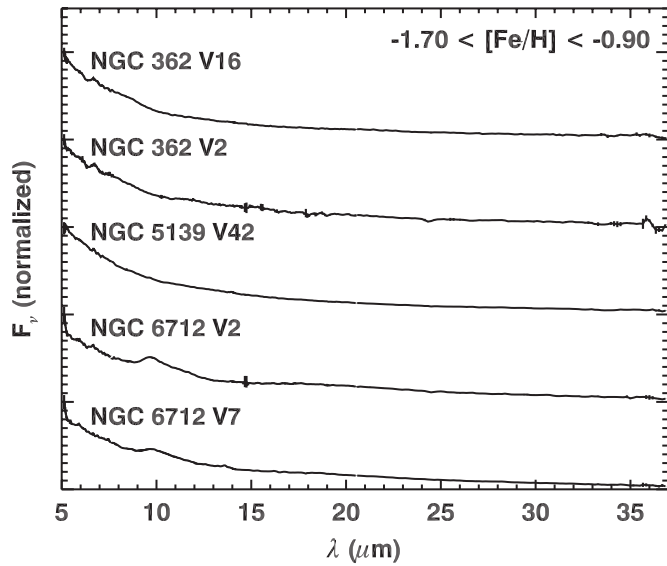
Figure 6. IRS spectra of the five AGB variables in our sample with metallicities ( [Fe/H] ) below -0.90 .
