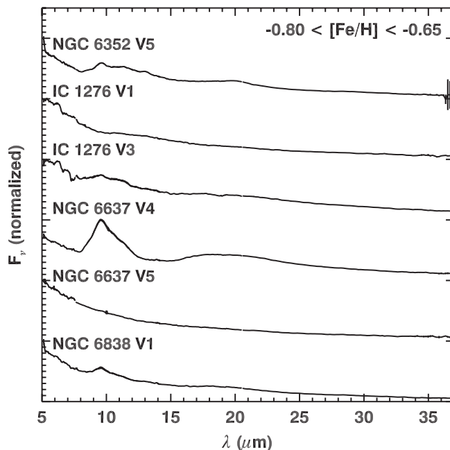
Figure 5. IRS spectra of the six sources in our sample with metallicities ( [Fe/H] ) from -0.65 to -0.80 .
