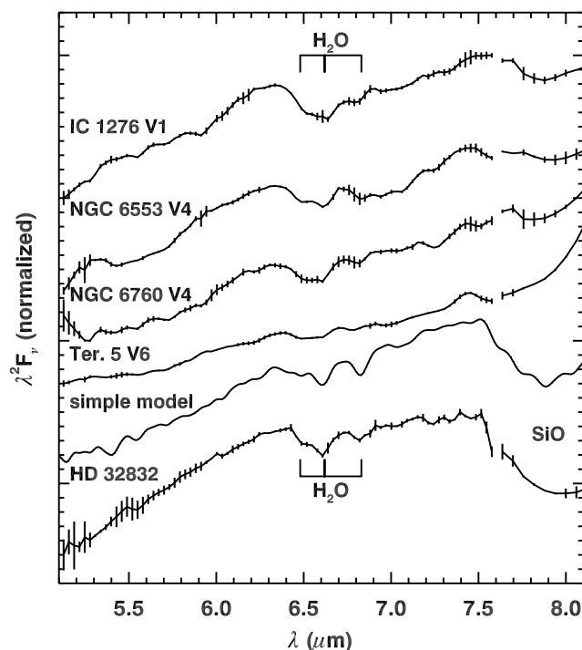
Figure 19. Four IRS spectra of globular cluster variables showing water-vapor absorption at 6.4\text{--}6.8\ \mu\text{m} , but no \text{SO}_2 absorption at 7.3\text{--}7.5\ \mu\text{m} , a simple model, and HD 32832, a naked Galactic comparison source with a spectral class of M4 III observed by the IRS. The spectra are plotted in Rayleigh–Jeans units as in Figure 18. The simple model only includes \text{H}_2\text{O} and SiO.
