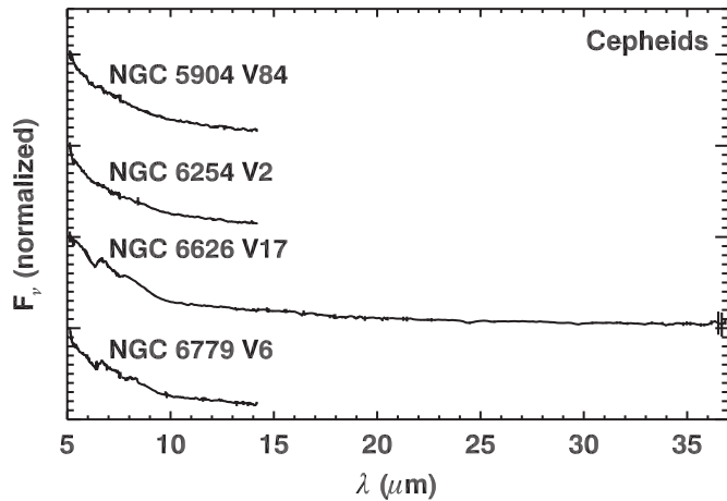
Figure 7. IRS spectra of the four Cepheid variables in our sample. All have metallicities ( [Fe/H] ) below -1.0 . Only one of the four has LL data.
