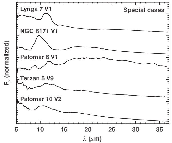
Figure 8. IRS spectra of the five sources which cannot be included in the metallicity-dependent analysis, as explained in Section 3.3.
