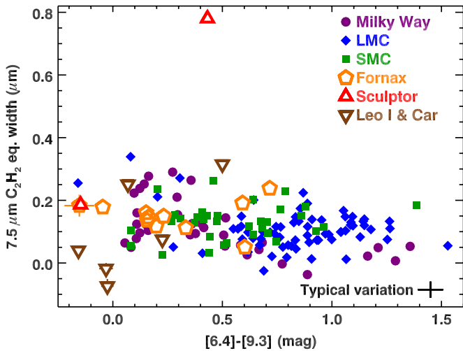
Figure 11. Equivalent width of the absorption band from C_2H_2 at 7.5 \mu m as a function of the [6.4]–[9.3] color. The data point in the top center is MAG 29 in Sculptor. This spectrum has a 7.5 \mu m band more than twice as deep as any other measured. The general trend of stronger absorption bands with decreasing metallicity is most apparent for 0.5 < [6.4]–[9.3] < 1.0 .
