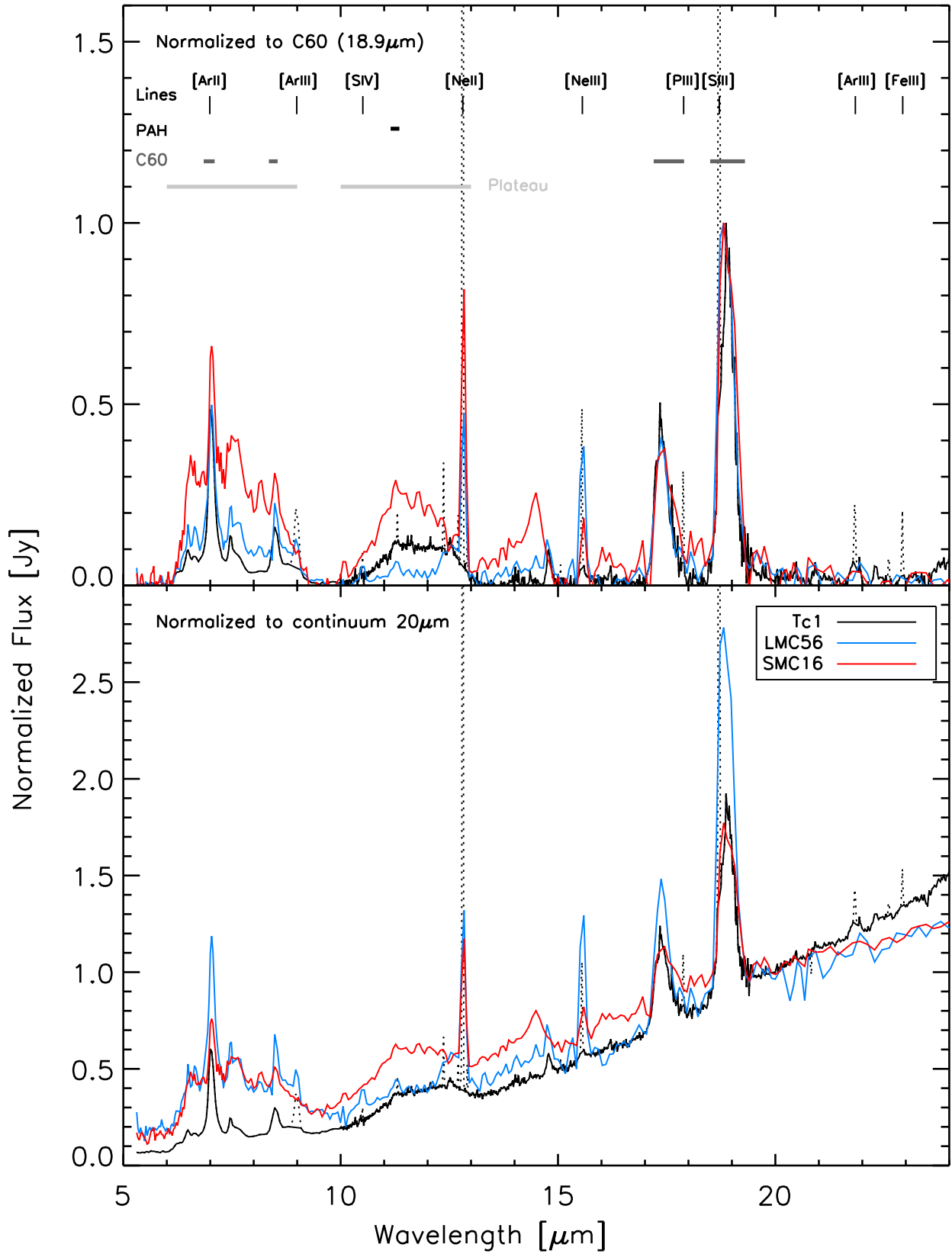
Figure 2. Top panel: Continuum subtracted spectra of the 5-24 \mu\text{m} region normalized to the peak of the 18.9\mu\text{m} feature. Atomic fine-structure lines in Tc 1 are shown as dotted lines. Bottom panel: Spectra normalized to the 20\mu\text{m} continuum flux. As can be seen the three PNe have very similar continuum emission.
