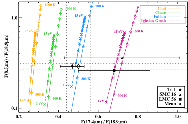
Figure 5. A diagnostic plot showing measurements and different model values for the total flux in the 8.5\ \mu\text{m} band and the flux in the 17.4\ \mu\text{m} band (both normalized to the 18.9\ \mu\text{m} band). Each pair of curves corresponds to a different source of C_{60} band strengths. The right hand curve for each pair corresponds to the band ratios for thermal models. The diamond plot symbols correspond to temperature increments of 100 K, and a low and a high temperature value is indicated on each curve. The left hand curves are model values for IR fluorescence. The crosses correspond to increments in the average absorbed photon energy of 1 eV. For each curve, the 1 eV and 15 eV models are indicated. We also show the measured band ratios for each of our three PNe, and the weighted mean value of the band ratios. The dotted lines indicate the 1\ \sigma confidence intervals for the mean values.
