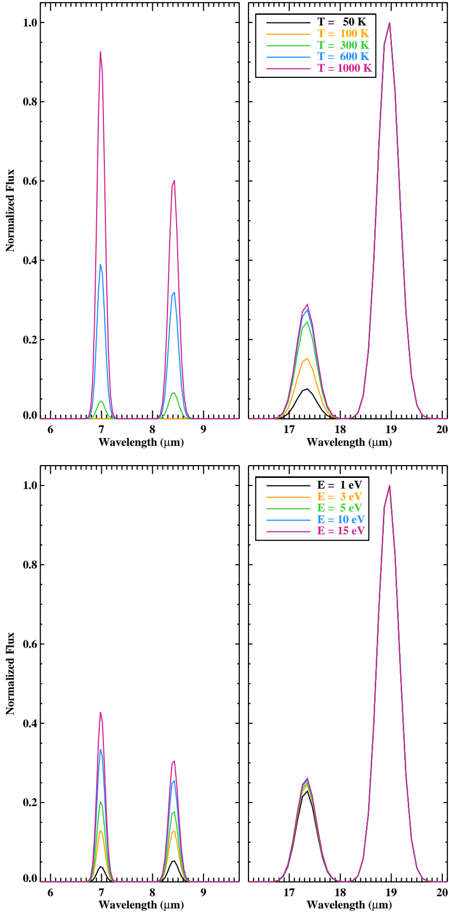
Figure 4. This figure shows how the relative strengths of the \text{C}_{60} bands changes as a function of temperature for thermal models (top) and as a function of the average absorbed photon energy for IR fluorescence models (bottom). In all cases, we used the intrinsic band strengths from Choi et al. (2000), and distributed the total power over Gaussian profiles whose width is set by the resolution (taken to be R = 90 ). All figures are normalized to the peak emission in the 18.9\text{ }\mu\text{m} band. Note that in the observations presented here, the bands at 17.4\text{ }\mu\text{m} and 18.9\text{ }\mu\text{m} are much broader than the instrumental resolution and thus these figures cannot be directly compared to the
