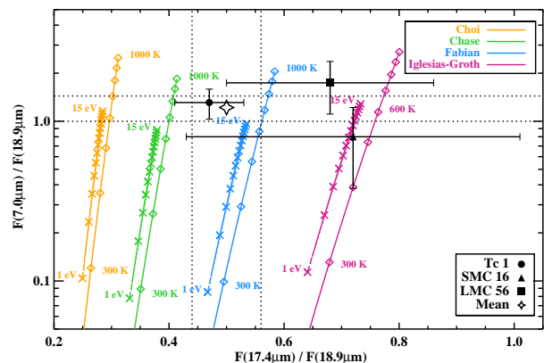
Figure 6. Same as Fig. 5, but for the 7.0\ \mu\text{m} band instead of the 8.5\ \mu\text{m} band.
