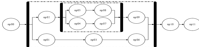
Fig. 3. Experiment service composition
