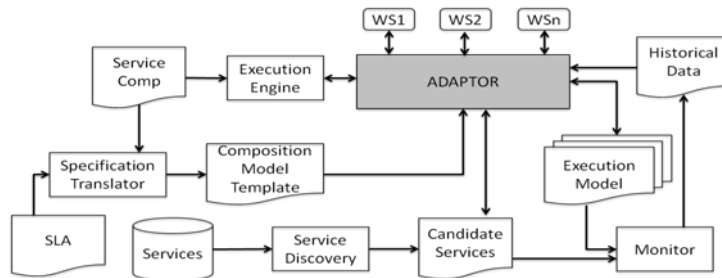
Fig. 1. ProAdapt architecture overview
