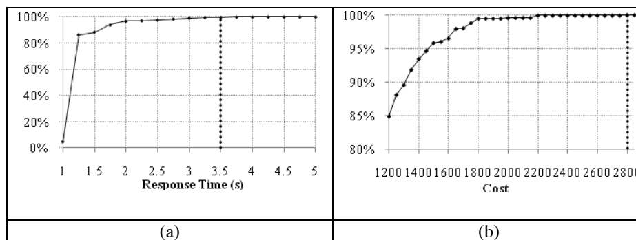
Fig. 7. Cumulative frequency distribution of (a) response times and (b) costs
