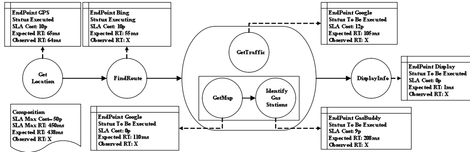
Fig. 2. Example of composition execution model
