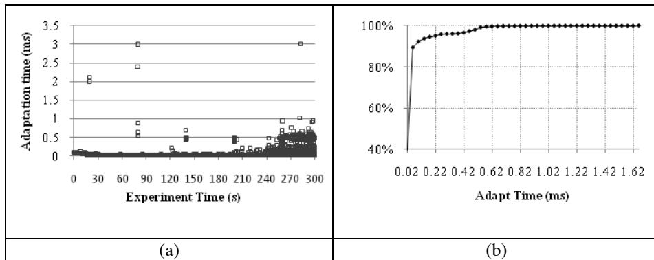
Fig. 8. (a) Adaptation time and (b) cumulative adaptation time over the experiment
