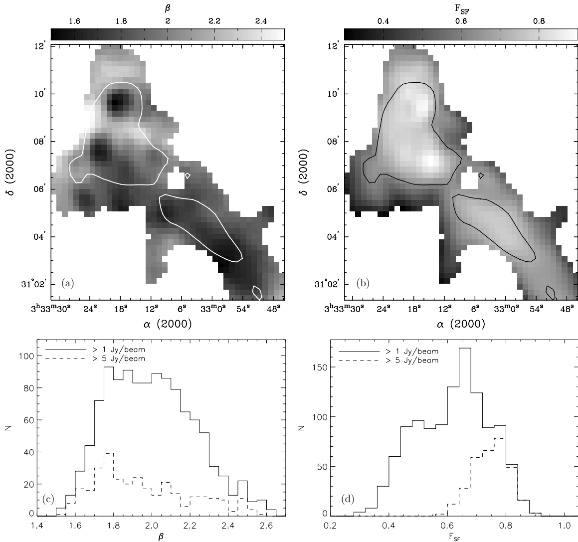
Figure 19. Top: results from the Spatial Factor Case highlighting (a) the dust emissivity and (b) spatial filtering factor ( F_{SF} ) for the emission (3), assuming an equal scaling factor, F_{SF} for the 450\ \mu\text{m} band and the 850\ \mu\text{m} band. The contours indicate the region with I_{450} > 5\ \text{Jy beam}^{-1} . Bottom: histograms for \beta and spatial filtering factor. The solid lines show the histograms for the entire region in the upper panels, and the dashed lines show the histograms for the I_{450} > 5\ \text{Jy beam}^{-1} regions, only. For these analyses, the 450\ \mu\text{m} data were scaled downward by 12.5% to account for the fractional increase in brightness in the observed maps over the predicted maps (see Figure 11).
