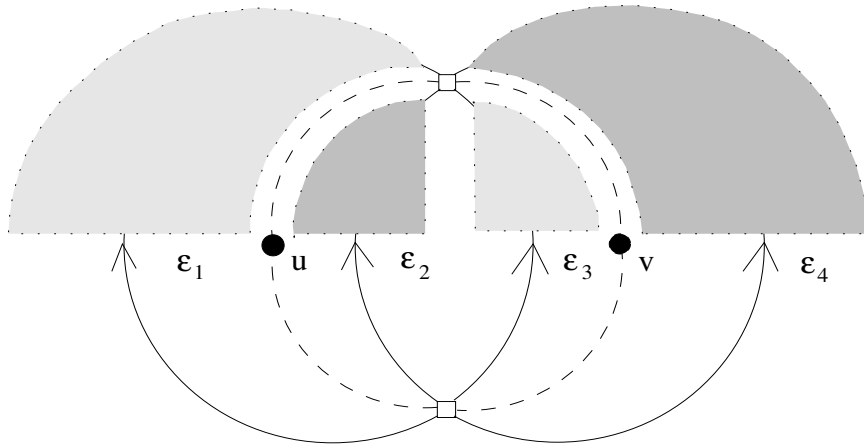
FIGURE 1. The two-vertex map M .
