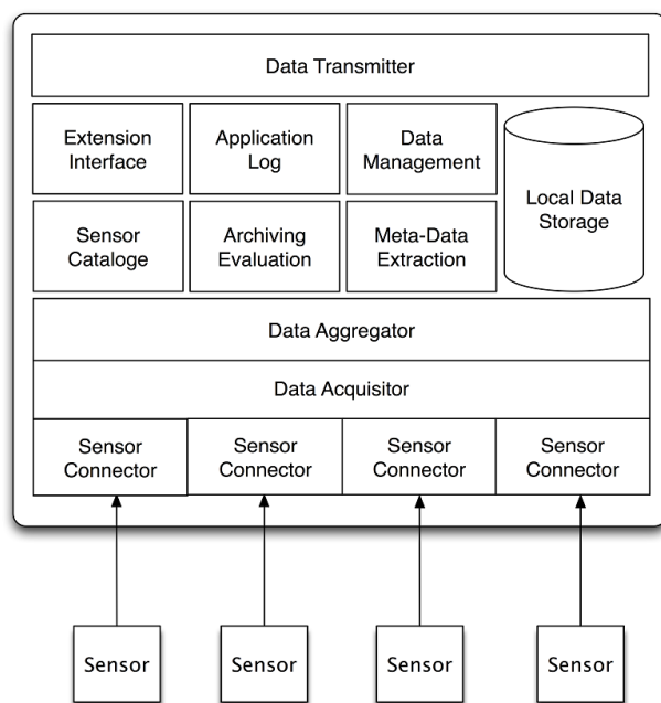
Fig. 2 UbiqLog Framework Architecture.
