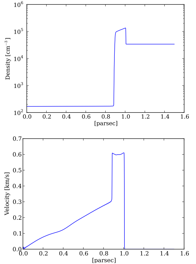
Fig. B.2. Density and velocity profile of a 1D spherical simulation of the ionization of a homogeneous medium in the conditions of RCW 36. The radius is between 0 and 1.5 pc with 2000 cells. The initial density is 3.4 \times 10^4 \text{ cm}^{-3} , the ionizing flux 6 \times 10^{47} \text{ ph s}^{-1} and the simulation is run during 720 ky.
