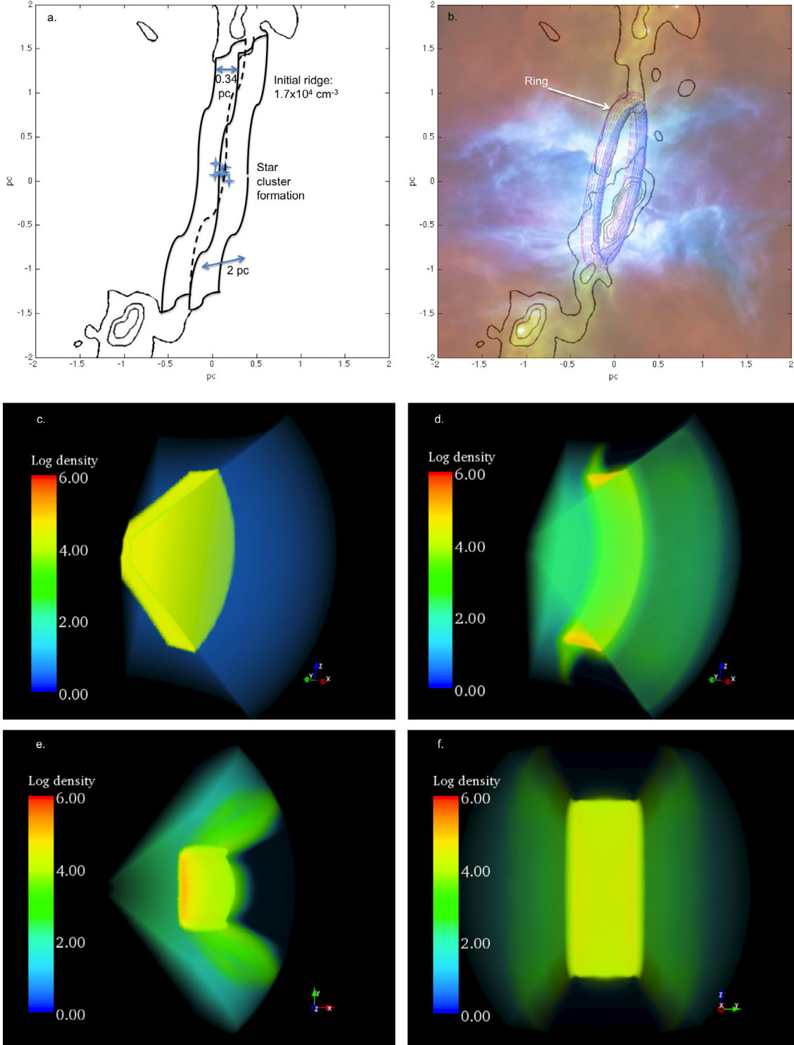
Fig. 5. Illustration of the proposed scenario. Observations: a) Schematic view of the initial ridge as derived in Sect. 3.2. b) Modelled ring superimposed on the Herschel 3-colour image. Numerical simulations: c) Cut through the plane of the initial ridge. The radius of the yellow circular section is 1 pc. The density is given in \text{H I cm}^{-3} . d) Cut through the plane of the ridge after ionisation reshaped it and formed a ring. e) Cut of d) from above. The bipolar shape clearly appears. f) Cut of d) from the backside. The ridge/filament projected shape clearly appears. The orientation of each cut is given by x , y , z axes on each image.
