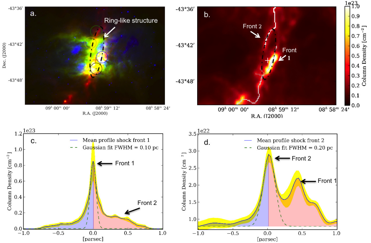
Fig. 2. a) Three-colour image of RCW 36 nebula (red: SPIRE 250 \mu\text{m} , green: PACS 70 \mu\text{m} , blue: \text{H}\alpha ). The cross indicates the ionizing source. Each coloured circle indicates area for which CS spectra have been integrated as in Fig. 7. The ellipse highlights the ring of compressed gas. b) column density map around RCW 36. The DisPerSe skeleton is drawn in white and each part of the shocked layer is labeled front 1 and front 2. c) Profile of the front 1 traced by DisPerSe on a Herschel +P-ArTéMiS column density map at 12'' resolution. d) Profile of the front 2 traced by DisPerSe on a Herschel column density map at 36'' resolution. The yellow shaded area represents the standard deviation of the profiles. The green-dashed curve is the Gaussian fit used to determinate the FWHM width.
