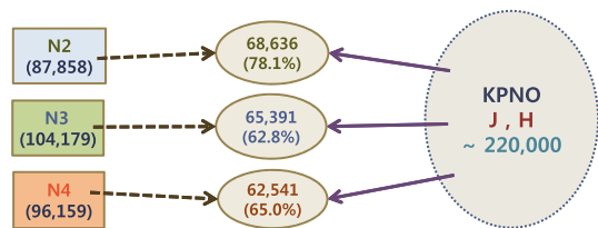
Fig. 18. Number of sources in each of the NIR band detection catalogs matched with KPNO J, H band data. About 78%, 63%, and 65% of the N2, N3, and N4 sources were found to have counterparts in the J and H band data.
