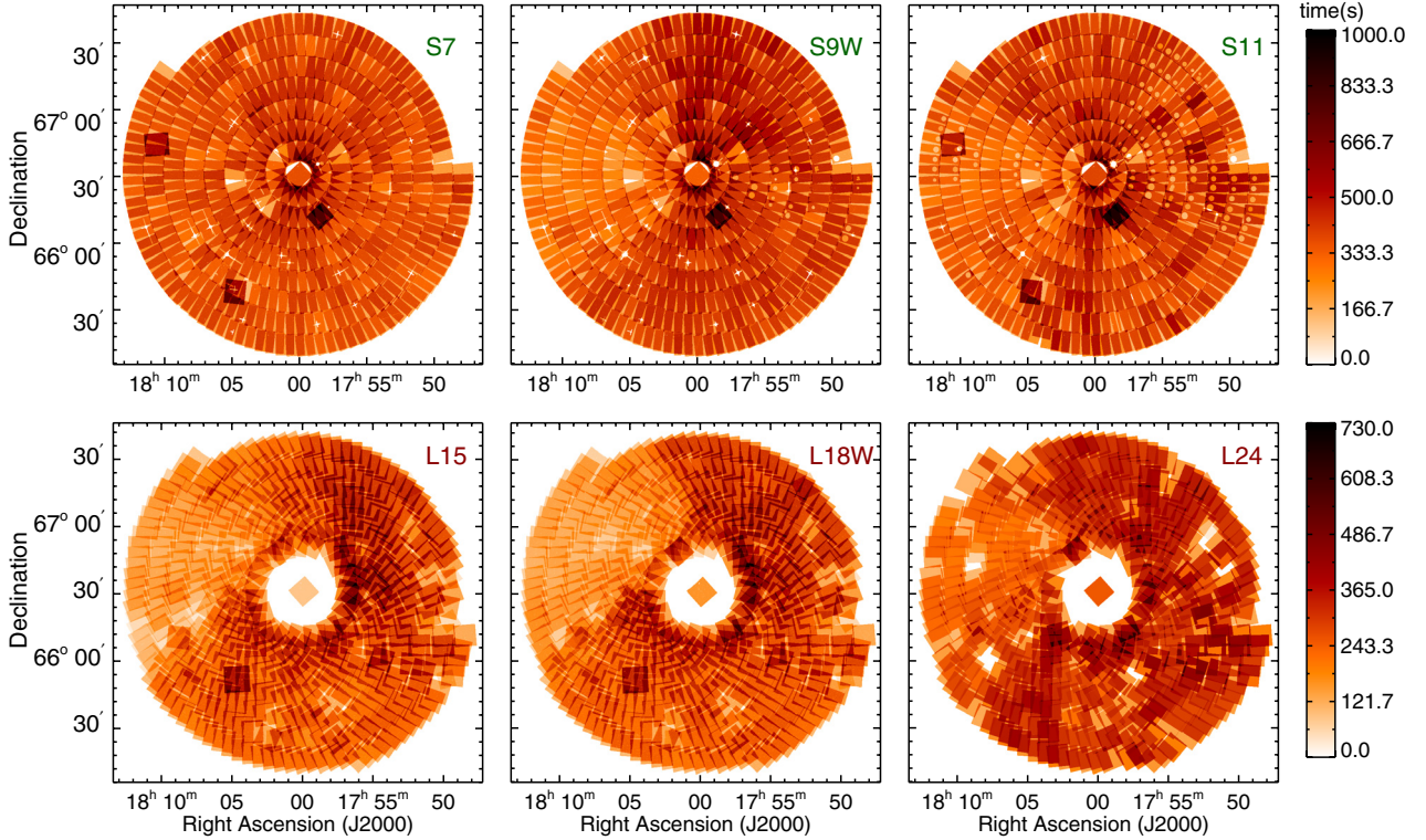
Fig. 10. Entire coverage maps of MIR-S ( upper ) and MIR-L ( lower ) bands.
