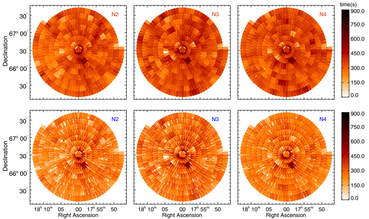
Fig. 9. Entire coverage maps of the NIR data before ( upper ) and after ( lower ) the correction for MUX bleeds. Uncovered area and none-weighted pixels have zero values (white area), which have wedge-like shape from the center to radially outer direction.
