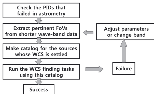
Fig. 4. Schematic flow chart describing the iterative procedures used to find a satisfactory solution for the WCS header of the L18W and L24 band data.
