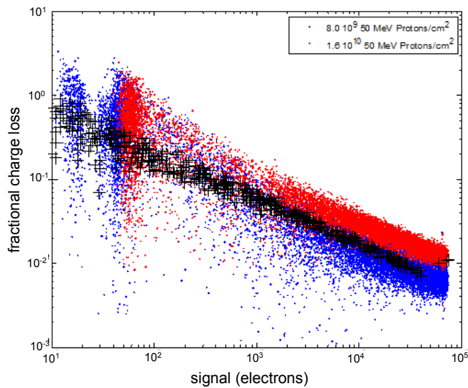
Figure 12. Plot of fractional charge loss measurements produced experimentally (dots) [15] with a charge injection delay of 200 ms, line dwell time of 2 ms and temperature of -130^{\circ}\text{C} for two different proton fluences. The simulated results (crosses, calculated for a mid-range fluence) are shown to demonstrate the same trend as the experimental data across all signal levels, demonstrating the consistency of this signal-volume methodology with the physical results provided experimentally [11].
