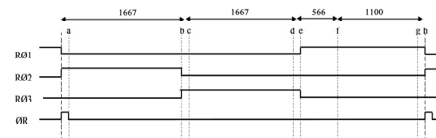
Figure 7. Burst mode and video mode clocking schemes as tested experimentally and subsequently simulated. The third scheme, “even mode”, was predicted to provide the best-case CTI following simulations, [12].
