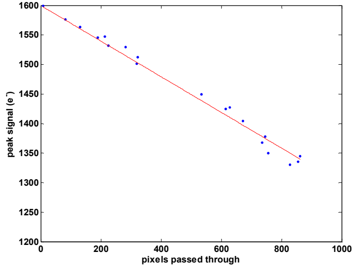
Figure 5. Plot of peak photon intensity versus position for Fe-55 X-ray events in the detector in photon counting mode. A best fit to the peak signal at positions across the CCD can be used to determine the CTI (here \sim 2 \times 10^{-4} ).
