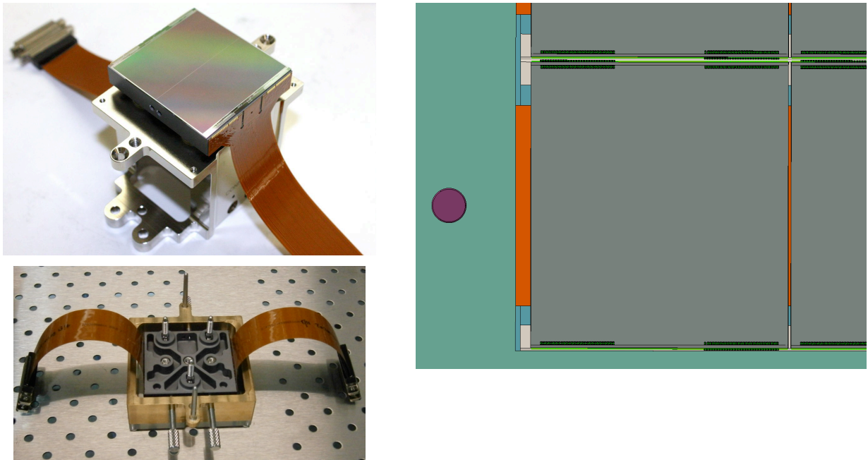
Figure 4: (left) The CCD273-82 to be used in VIS. A view of the active surface (top) shows the arrangement of the flexible connectors to allow close buttability. This is a front-illuminated variant for initial testing, so the charge injection structures are visible down the centre of the device: the devices used in flight will be back-illuminated. The rear surface (bottom) shows the SiC packaging. (Right) The layout of the CCD detector matrix on the FPA.
