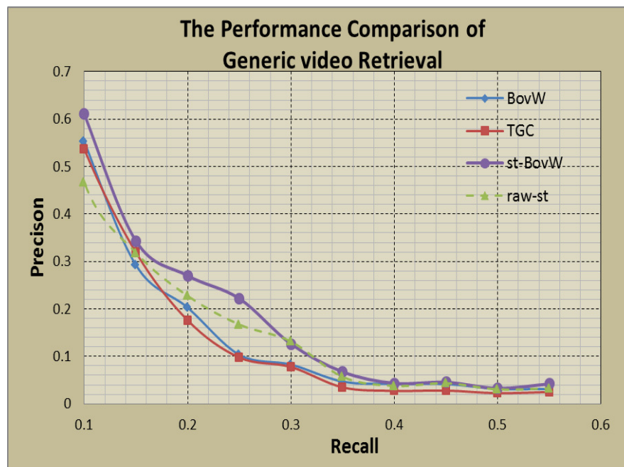
Figure 7: Precision-Recall curve for queries for Generic Video Retrieval
