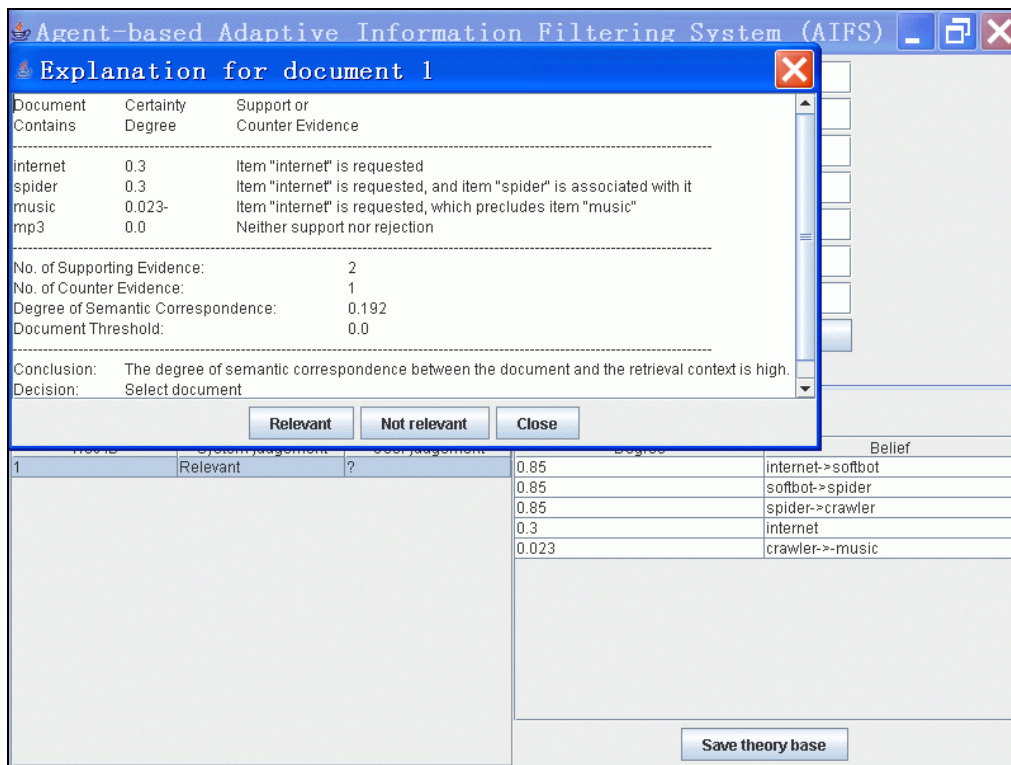
Figure 3 – Explaining the System’s Document Selection Decision
