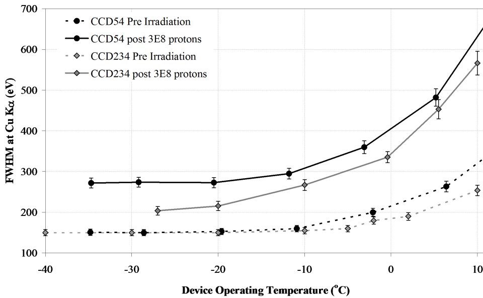
Fig. 6. Energy resolution measured using the Cu-K \alpha X-ray peak as a function of temperature for the CCD54 and CCD234 pre and post irradiation
