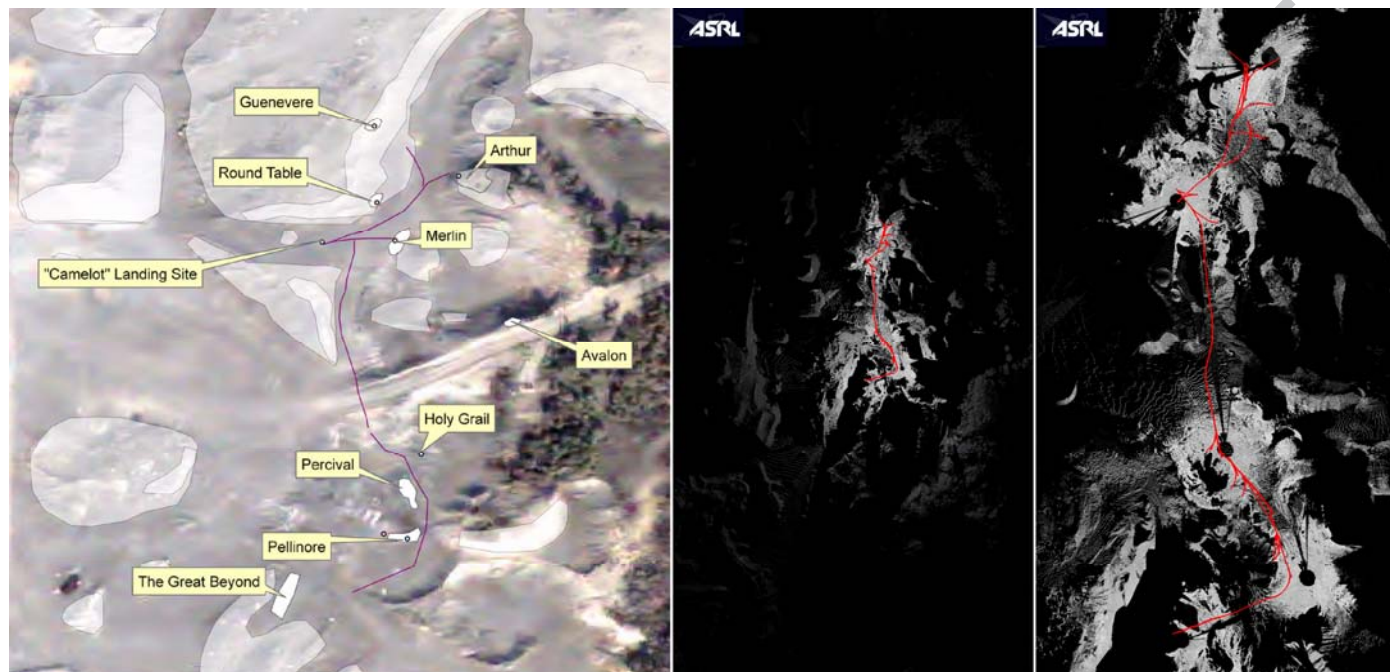
Figure 10 – a map of our traverses in Sudbury. (LEFT) A QuickBird satellite image annotated by the science team to highlight targets of interest. The rover network is highlighted in purple. (CENTRE, RIGHT) Two zoom levels of the LiDAR map acquired. The rover network is highlighted in red with each dark circle representing a new map centre that was stitched onto the whole. The total odometry is 2.20 km and includes one traverse which caused the rover to stop at the edge of a steep drop-off (furthest point towards feature “The Great Beyond” note the dark shadow on the LiDAR map) Another point of interest, shown in the upper right of the rightmost panel was selected due to its high elevation in order to acquire data at long range.
