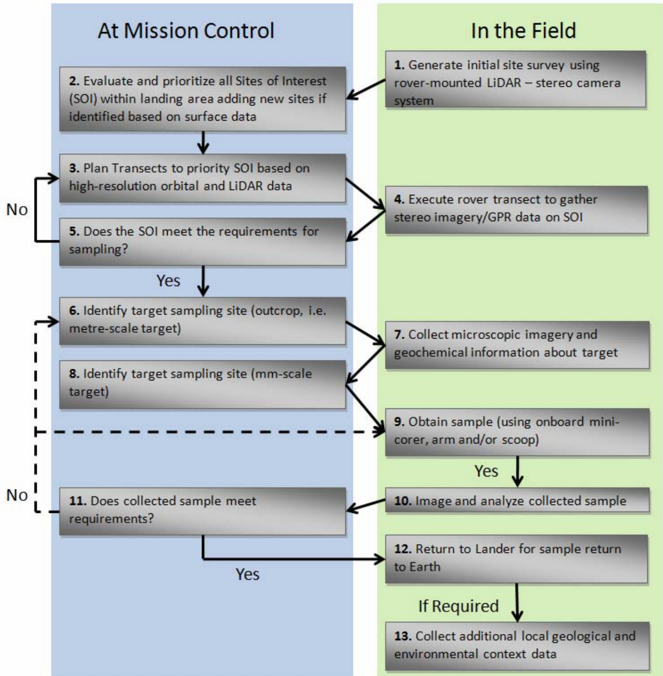
Figure 3 – The Sampling flowchart for the ILSR mission following landing, after Osinski et al., 2009. While this flowchart is written in the context of the investigation of a single Site Of Interest (SOI) to acquire a single sample, the ROC-6 roving network architecture allows this flowchart to be followed for several sites in parallel.
