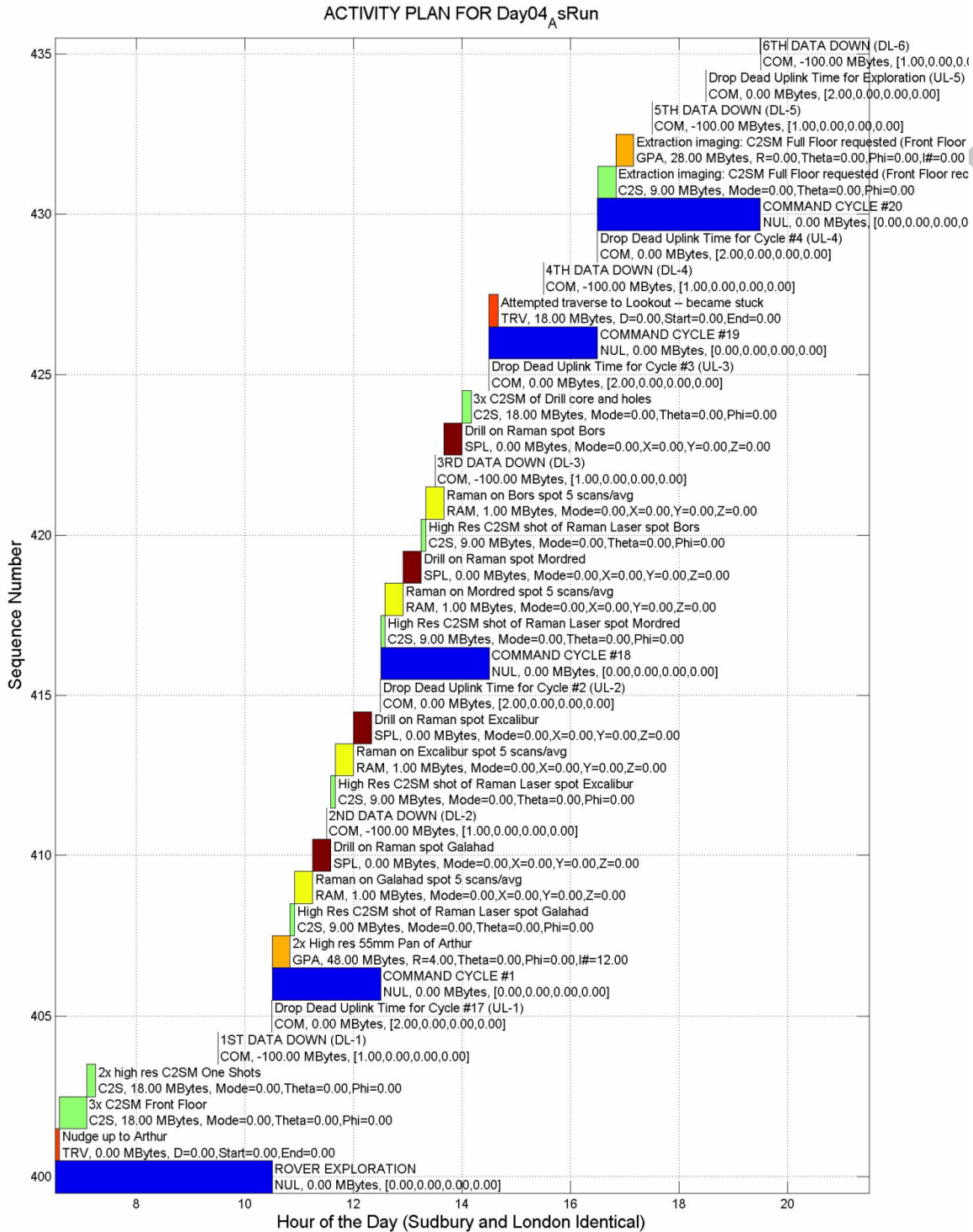
Figure 9 – A typical day’s plan as expressed in LASPI (Lunar Analogue Science Planning Interface). LASPI was a scheduling and resources tool employed by the SPIs within the Planning Process and was the chief high-level method of recording what activities were performed. Activities flow from bottom left to the upper right. Day 4 includes a nudge up to the “Arthur” outcrop, Raman analyses of coring sites and sample acquisition. An attempted traverse in Command Cycle 19 to get close to a second outcrop “Guinevere” was unsuccessful. Extraction Imaging in Command Cycle 20 was key to determining the reason for this fault.
