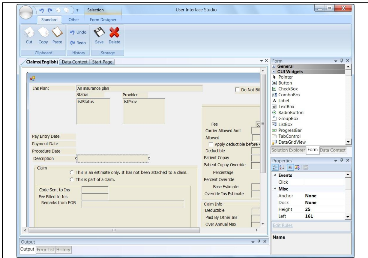
Figure 2: Our Concrete User Interface Designer
