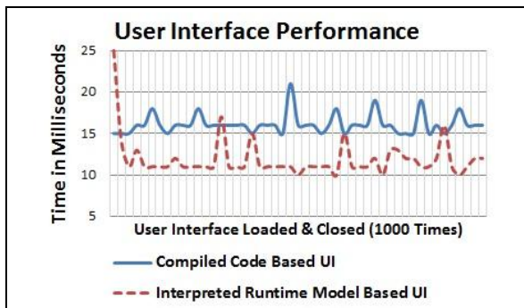
Figure 3: User Interface Performance
