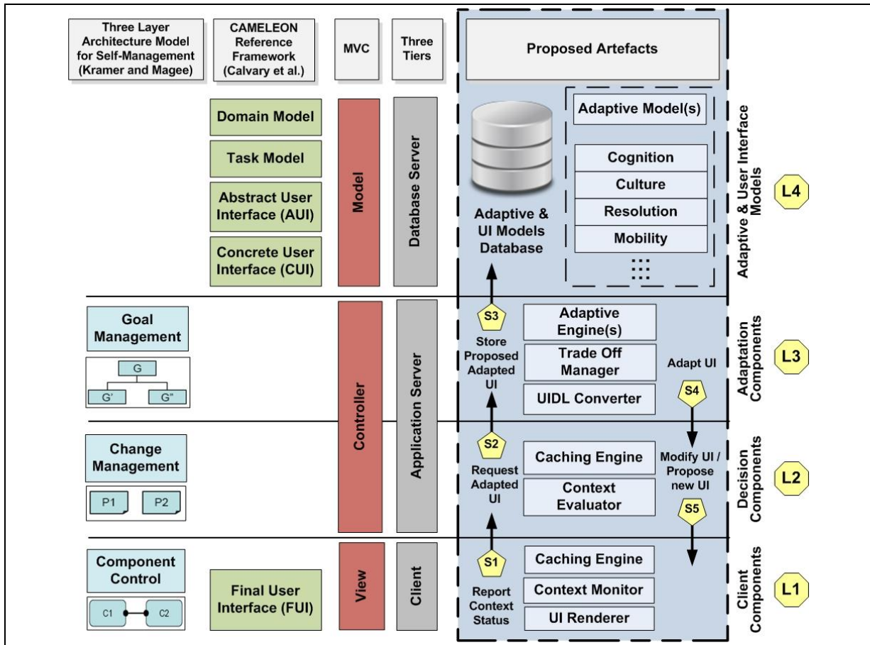
Figure 1: Proposed Architecture for Adaptive User Interfaces
