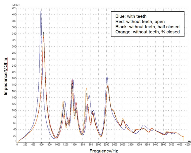
Figure 4: Input impedance magnitude curves for Howarth oboe with standard C7 fingering applied together with different degrees of venting.
