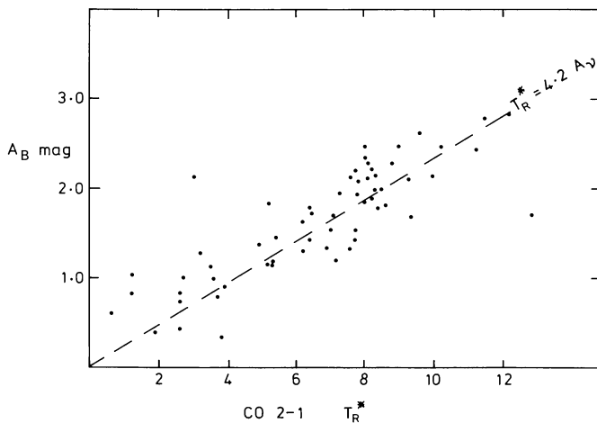
Fig. 7. Variation of T_R^* (K) width with A_B (magnitudes). A best-fit with T_R^* = \sim 4.2 A_B is found
