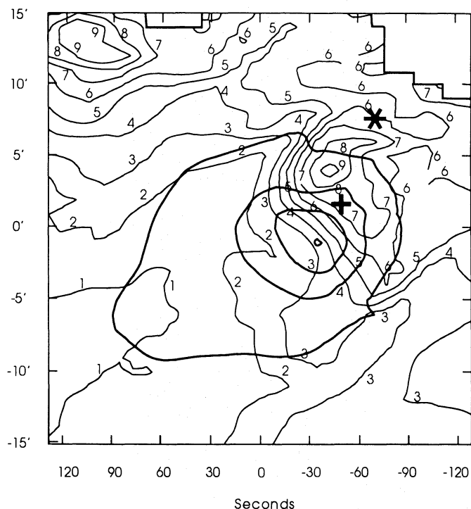
Fig. 6. Isophotal contour map of the 100- \mu\text{m} optical depth (thick lines) overlaid on the dust colour temperature (thin contours), calculated from the 60 and 100 \mu\text{m} flux densities. The optical depth contours are at 0.004, 0.01, 0.015 and 0.023; the dust colour temperature base level contour is at 31K and the contour interval is 2K. The (0,0) position is the same as for Fig. 5. The position of peak far-IR emission, R.A. (1950) = 22^{\text{h}}55^{\text{m}}08^{\text{s}} and Dec. (1950) = +62^{\circ}21'30'' , is marked with a cross and the position of the O7 star HD 217086 is marked with an asterisk
