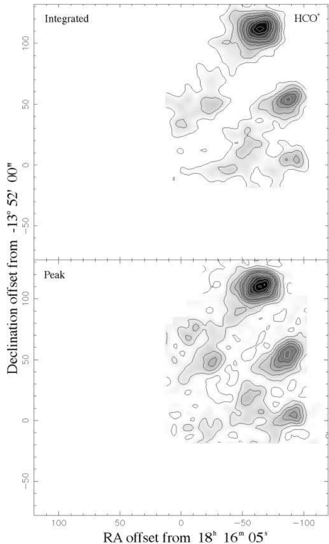
Fig. 11. \text{HCO}^+ J=4-3 integrated and peak and intensity maps over the range 20-28 \text{ km s}^{-1} . The lowest contour on the the integrated map is at 2 \text{ K km s}^{-1} , and the contour intervals are at 2 \text{ K km s}^{-1} intervals, and on the peak map is T_{mb} = 1.0 \text{ K} , and the contour intervals are at 0.75 \text{ K} intervals.
