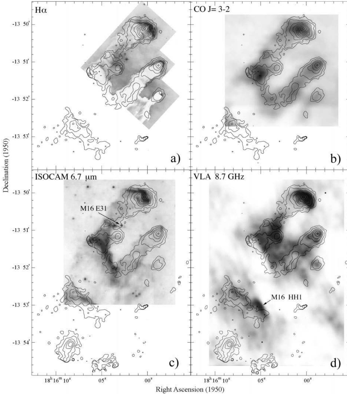
Fig. 2a–d. The SCUBA 450 \mu m map shown as contours, overlaid onto a the HST H \alpha image of Hester et al. (1996), b the CO J= 3-2 integrated emission, c the ISOCAM 6.7 \mu m image, and d the 8.7 GHz image. The contour levels on the 450 \mu m map are 5, 10, 20, 30, 40, 50, 60, 70 and 80 mJy per beam. The lower part of the SCUBA map is omitted from panels a and b , but included in the lower panels . M16 E31 is a bright IR source seen in the ISOCAM images of Pilbratt et al. (1998), and M16 HH1 is an Herbig-Haro object.
