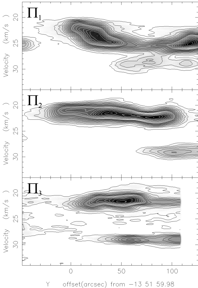
Fig. 8. Position velocity maps in the CO J=3-2 transition along the major axis of the three fingers. These plots were made by rotating the map 42.2 degrees in an anti-clockwise direction, then integrating along the major axis of the fingers, with a 40'' slit centred on the axis of the finger. The tips of the fingers appear on the right hand side of these plots.
