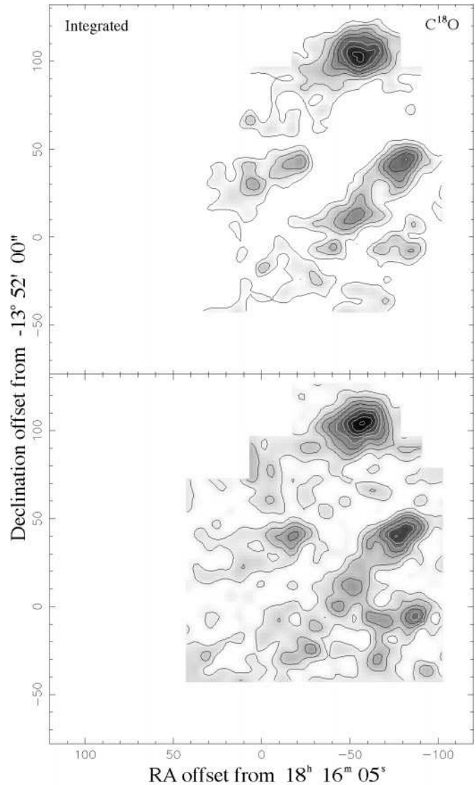
Fig. 9. \text{C}^{18}\text{O} J=3-2 integrated and peak intensity maps integrated over the velocity interval 20-28 \text{ km s}^{-1} . The lowest contour level shown on the integrated map is at 2.3 \text{ K km s}^{-1} , and the contour is spaced at 2.3 \text{ K km s}^{-1} intervals. On the peak map the first contour has a value of 2.3 \text{ K} , and the contours are spaced at 1.15 \text{ K} intervals.
