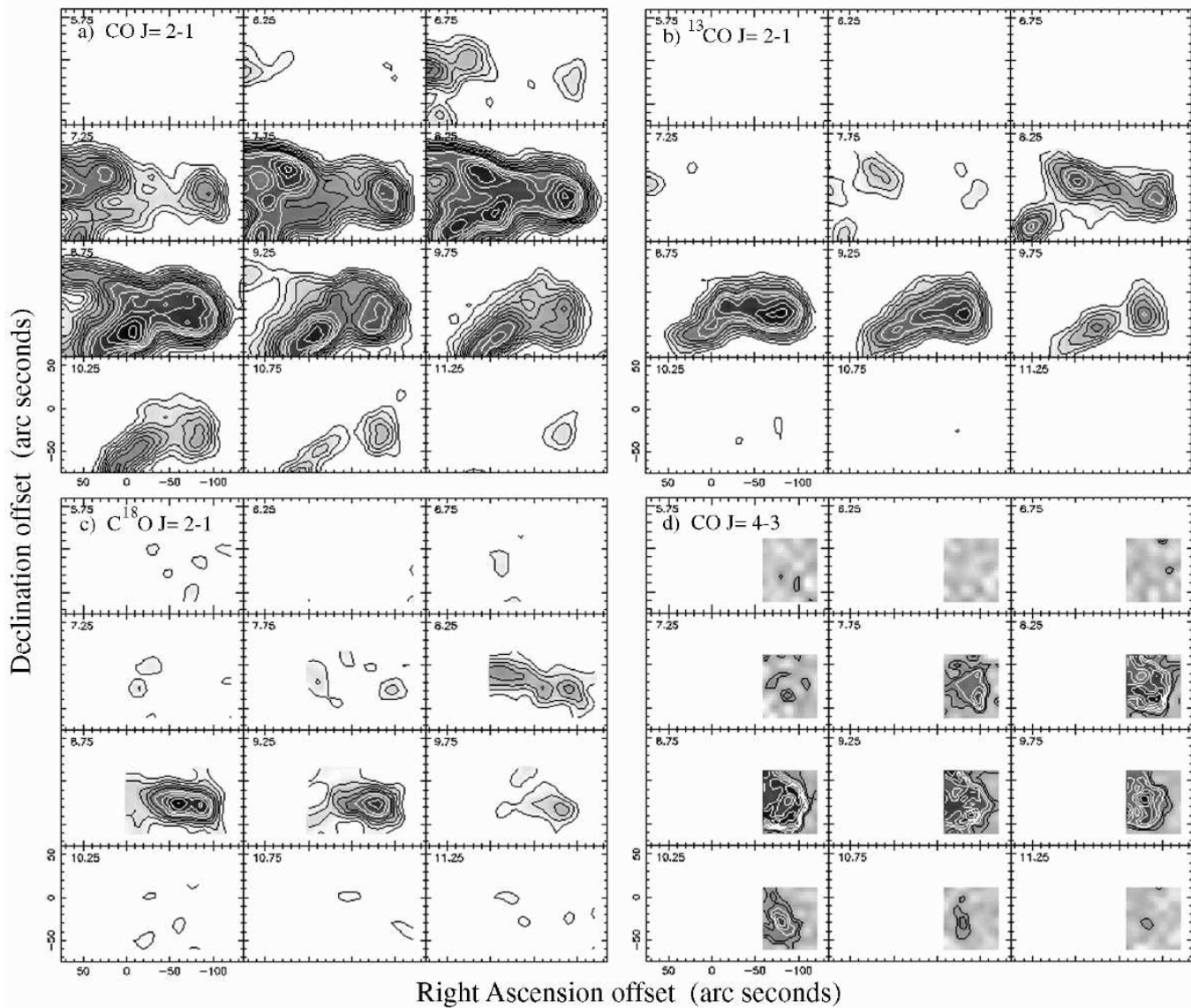
Fig. 5a–d. Channel maps at 0.5 \text{ km s}^{-1} intervals for a \text{CO } J = 2 - 1 (with the first white contour at 4.7 \text{ K km s}^{-1} and contour intervals at 0.9 \text{ K km s}^{-1} ), b ^{13}\text{CO } J = 2 - 1 ( 3.4, 0.43 \text{ K km s}^{-1} ), c \text{C}^{18}\text{O } J = 2 - 1 ( 1.2, 0.2 \text{ K km s}^{-1} ) and d \text{CO } J = 4 - 3 ( 4, 1 \text{ K km s}^{-1} .)
