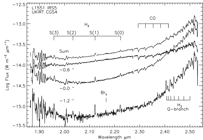
Fig. 22. UKIRT archive spectrum towards L1551 IRS 5. This intensity at the (0,0) position is about three times weaker than the Carr et al. spectrum – but in reasonable agreement since the emission is extended relative to the UKIRT beam.
