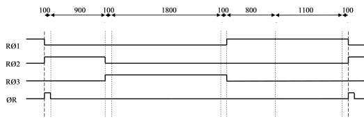
Fig. 2. The 'video mode' clock timing diagram as sequenced, with times shown above the scheme in nanoseconds. Two equal pulses are implemented at 2 \mu\text{s} each followed by a single pulse at 1 \mu\text{s} . [5]
