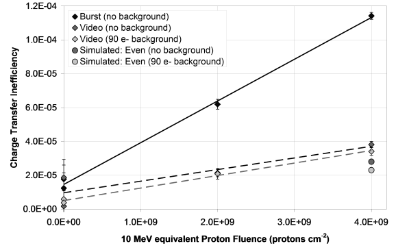
Fig. 7. The experimental data for the two clocking schemes described previously are shown in comparison to the simulated results for the proposed optimised clocking scheme. The CTI has been calculated from a signal of approximately 1600 electrons ( \text{Mn-K}\alpha ) in both the experimental and simulated results, with both low and 90 e^- background included. With no background, the ‘even clock spacing’ scheme (Figure 6) was simulated to have a CTI level 2.8 \times 10^{-5} , an improvement of approximately 26% [3].
