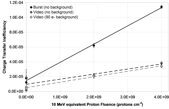
Fig. 5. The serial CTI, measured using Mn-K \alpha X-rays at a signal level of approximately 1600 e - as a function of 10 MeV equivalent proton fluence. Results are shown with and without an optical background of approximately 90 e - [5].
