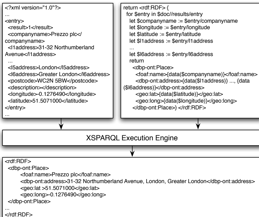
Fig. 3. An example for preparing the service request.
