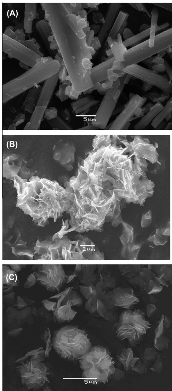
Fig. 2. SEM images of hydrous magnesium carbonate phases precipitated during this study: Nesquehonite needles collected from (A) experiment Bio-A after \sim 1 h, (B); dypingite rosettes collected from experiment Bio-A after 30 days, and (C) Abio-A after 27 days.
