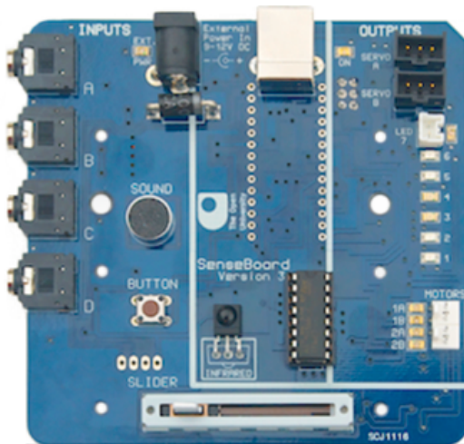
Figure 1: The SenseBoard
