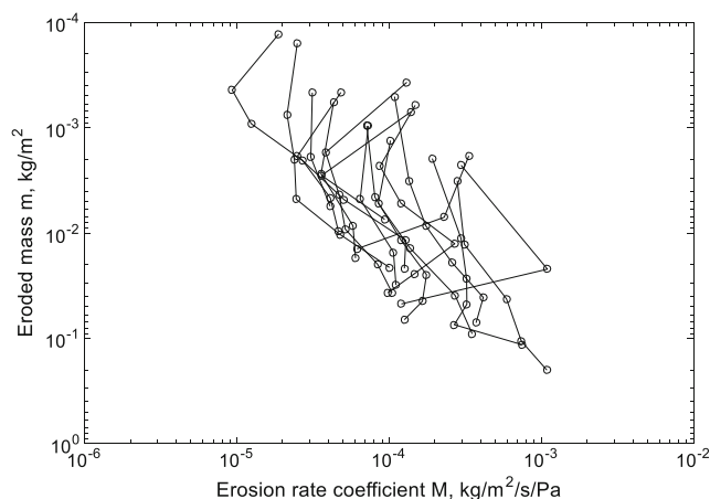
Fig. 5 Erosion rate coefficient computed from erosion microcosm data for 15 cores from Franks Tract. The vertical axis of eroded mass increases down the page to mimic depth dependency
