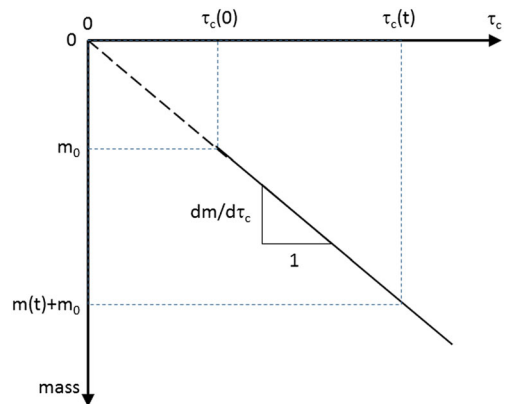
Fig. 10 Eroded mass and critical shear stress \tau_c are assumed to be linearly related with a slope of dm/d\tau_c . Initial critical shear stress \tau_c(0) corresponds to an initial eroded mass m_0 such that if \tau_c(0) was zero, the eroded mass would be zero. At time t , the mass eroded during the experiment is m(t) and the critical shear stress is \tau_c(t)
