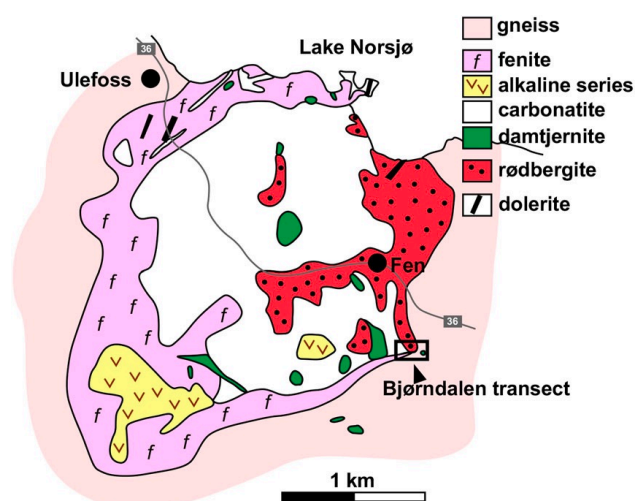
Figure 1. Simplified map of the Fen Complex, based on NGU map ( geo.ngu.org ) and our own data. Our key sampling transect is marked in box. Rødbergites, i.e. strongly REE-enriched secondary hematites are highlighted.
