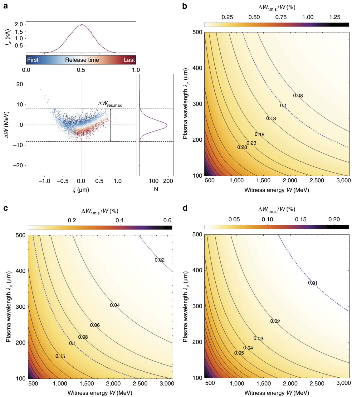
Figure 5 | Residual energy spread from simulation and scaling prediction. Absolute residual witness energy spread from simulation ( a ) and relative energy spread from scaling predictions ( b–d ). In ( a ), the residual energy spread as observed in the PIC-simulation at minimum energy spread position (corresponding to the case depicted in Fig. 3c) is shown with color-coding of laser-released witness electrons, where position 0 indicates the first electron released and position 1 indicates the last electron released. Electrons which are released earlier (blue) are gaining more energy than those released later (red), in accordance with the numerical scaling estimation. b–d show relative energy spread predictions based on the residual energy spread scaling for a witness release laser spot size of w_{0,w} = 10 \mu\text{m} ( b ), w_{0,w} = 7 \mu\text{m} ( c ) and w_{0,w} = 4 \mu\text{m} ( d ) in dependence of witness bunch energy and wavelength of the accelerating plasma wave. Isolines depict the combinations of constant relative energy spread for selected values.
