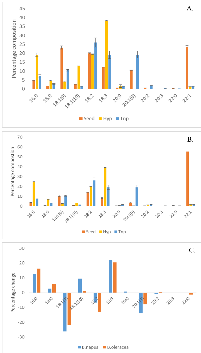
Figure 25. Fatty acid composition of Brassicac tissues, A – Brassica napus . B – Brassica oleracea . C – Percentage change in Fatty acid composition between seed and adult hypocotyl. Values calculated from 3 biological repeats Error bars represent +/- 2SE.
