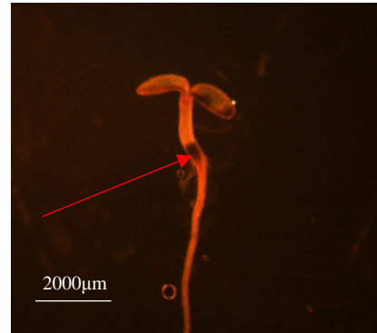
Figure 7 7 day old tnp seedling grown on \frac{1}{2} MS 30 & 10nm 2,4D stained with Lugol solution. Arrow indicates a strong presence of starch within the hypocotyl which is indicative of the tnp phenotype.
