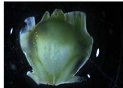
Figure 17 5 week old B.oleracea stained with Lugol for starch showing significantly less staining than the other Brassic as at the same time point.
