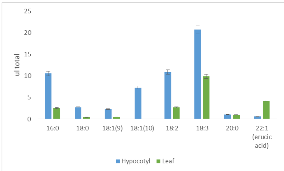
Figure 24 Fatty acid composition of Brassica tissue, 1g used for each reaction, 100mg used for GC run. A – Brassica napus hypocotyl vs Brassica napus leaf. B – B.napus & B.rapa profiles. Values calculated from 3 biological repeats Error bars represent +/- 2SE.
