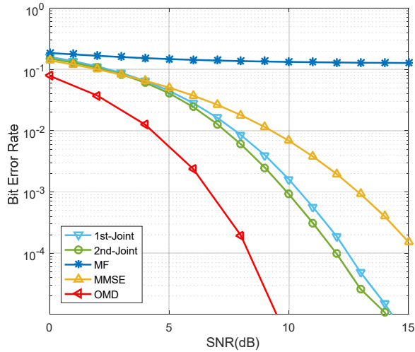
Fig. 10. BER performance of dupe joint detection method with user number K=50 .
