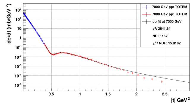
Fig. 4 The pp elastic scattering model model fit (fitted over all data) shown for \sqrt{s} = 7000 GeV, over the full published t range
