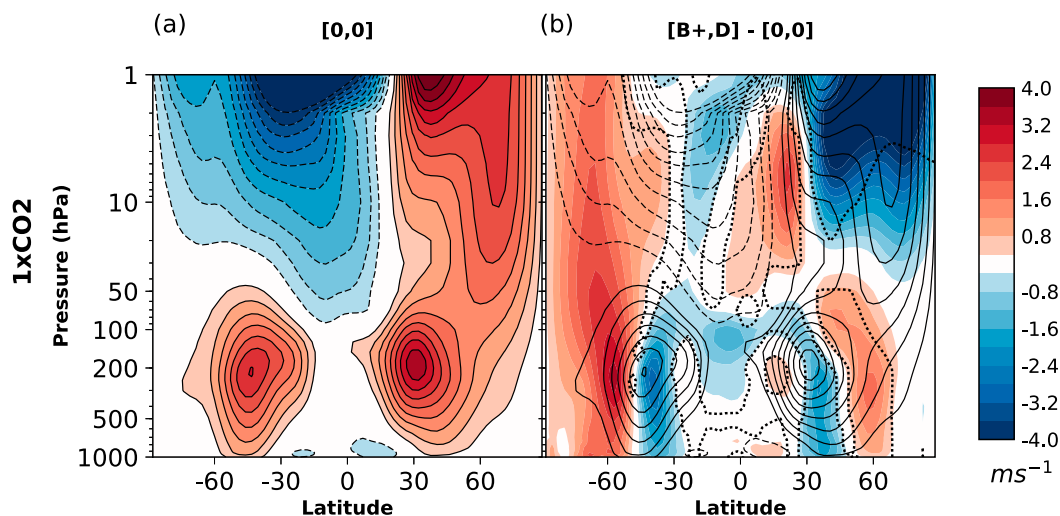
FIG. 2. DJF [u] . (a) The [0, 0] 1\times\text{CO}_2 climatology; contour interval is 5\text{ m s}^{-1} . (b) Line contours indicate [0, 0] climatology, and colored contours are the response to drag ( [B+, D] minus [0, 0] ), with contour interval given by the color bar. Regions of statistically significant differences (at the 95% level based on the two-sided independent Student's t test) are encompassed by dotted black lines, as is also the case in subsequent figures.
