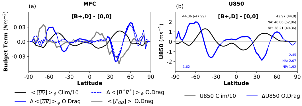
FIG. 1. (a) DJF 1 \times \text{CO}_2 MFC climatology divided by 10 (solid black line) and response to parameterized orographic drag (solid blue line). The solid gray line is the zonal-mean total (freely propagating, blocking, and downslope wind) parameterized orographic stress F_{OD} at 1 \times \text{CO}_2 . The dashed blue line is the SEMFC response to drag. (b) DJF 1 \times \text{CO}_2 u 850-hPa climatology divided by 10 (solid black line) and response to drag (solid blue line). See text for description of values quoted in (b). Regions of statistically significant differences (at the 95% level based on the two-sided independent Student's t test) are indicated by a thickening of the line.
