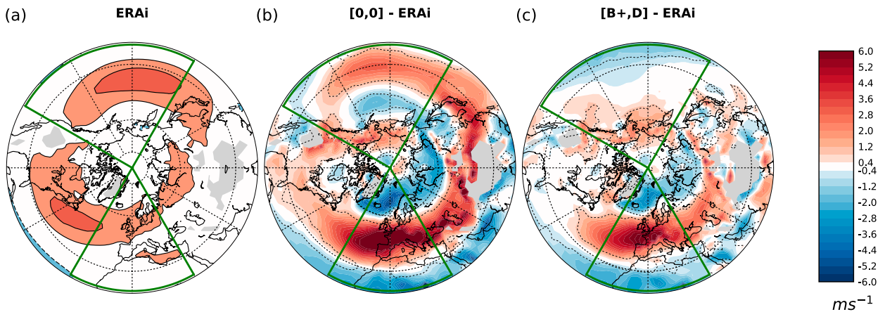
FIG. 4. DJF u 850 hPa. (a) ERA-Interim climatology, contour interval is 5 \text{ m s}^{-1} . (b) [0, 0] minus ERA-Interim. (c) [B+, D] minus ERA-Interim. Contour interval in difference plots given by the color bar.
