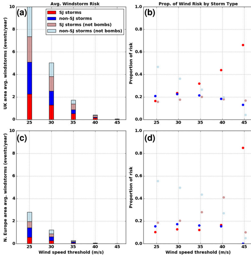
FIG. 11. (a) Frequency (events \text{yr}^{-1} ) of strong resolved wind events in storms with (red shading) and without (blue shading) sting-jet precursors averaged over the U.K. domain (marked in Fig. 10) for resolved wind speed thresholds from 25 to 45 \text{m s}^{-1} (increment 5 \text{m s}^{-1} ). Distinction is made between storms that did (dark shading) and did not (light shading) develop explosively. (b) As in (a), but data plotted as a proportion of total frequencies for each resolved wind speed threshold. (c),(d) As in (a),(b), but for the continental western European domain (marked in Fig. 10). Some of the points in (b) and (d) are displaced slightly from the resolved wind speed threshold lines for clarity.
